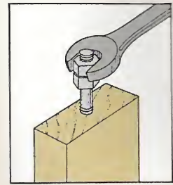
To insert a hanger bolt, thread two nuts on the shaft and tighten them together. Then use a wrench to screw the bolt in.
