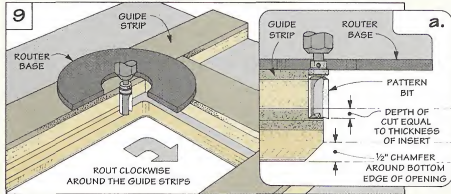
▲ Using a pattern bit in a router is a quick way to rout the recessed lip in the top. The bearing on the pattern bit rides against guide strips and cuts a recess exactly the same size as the insert plate.
