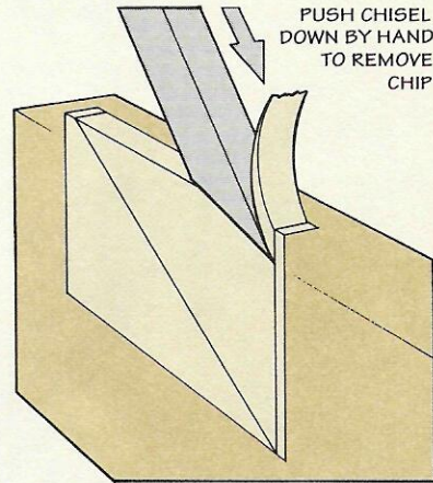
Step 2. With the bevel down, remove a chip. To prevent crushing the ends of the mortise, leave \frac{1}{8} " at each end of the mortise.
