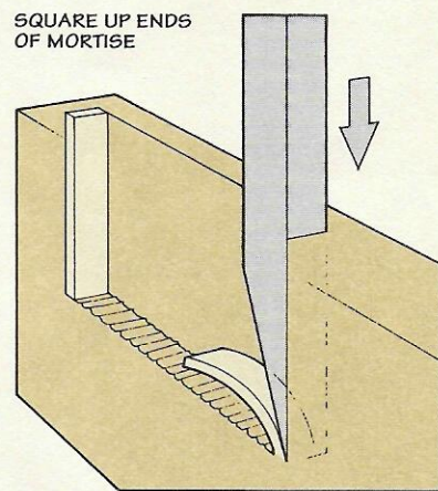
Step 5. Finally, to complete the mortise, pare away the \frac{1}{8} " section that you left at each end of the mortise.
