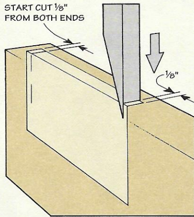
Step 1. With the flat of the chisel toward the end of mortise, use a mallet to drive the chisel vertically into the wood about \frac{1}{4} ".
