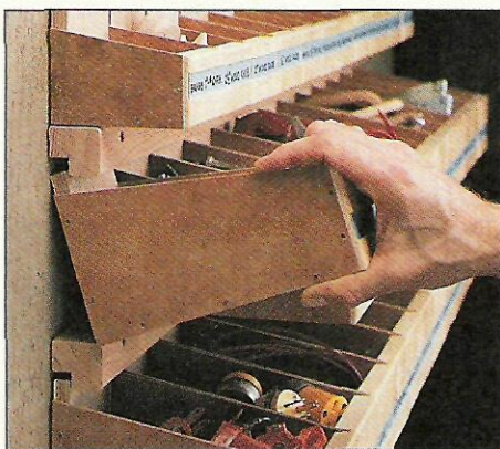
▲ The back of each bin “locks” into a wall-mounted rail. To remove the bin simply lift the front up and pull it out.
