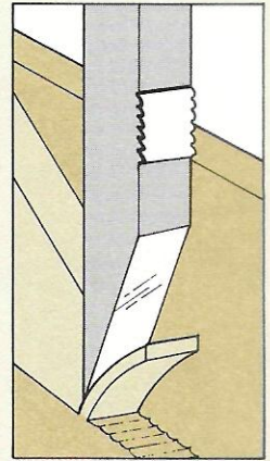
Stick a piece of tape on the chisel to act as a depth gauge.
