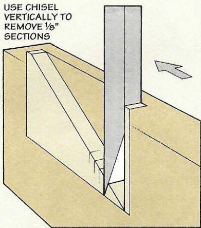
Step 3. To clean out the remaining waste, hold the chisel with the bevel toward the low end of the ramp and chisel out \frac{1}{8} " sections.
