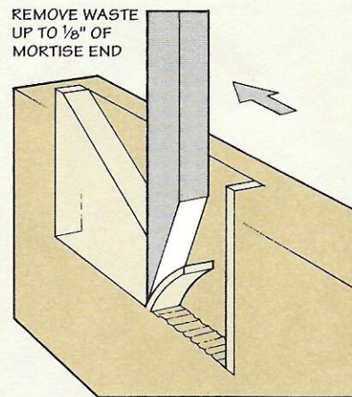
Step 4. Continue in this manner for the entire length of the mortise. Taking \frac{1}{8} " cuts and prying out the waste.
