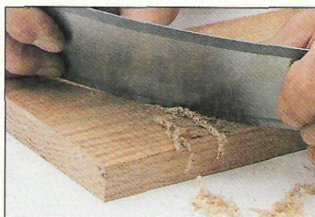
▲ Planer Marks. Hand scrapers can be used to quickly remove the ridges or marks left by a planer.
