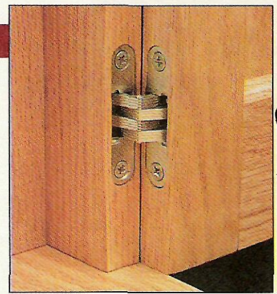
▲ The laminated links of this Soss Invisible Hinge slide inside the body. This conceals the hinge when it's closed.
