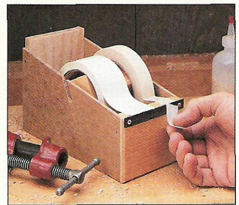
▲ This tape dispenser is another handy accessory. It’s just a storage bin with a few modifications.
