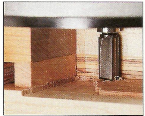
Hinge Mortising Jig page 4
