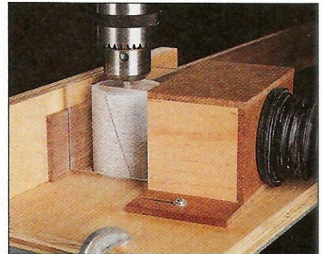
Thickness Sanding Jig page 8
