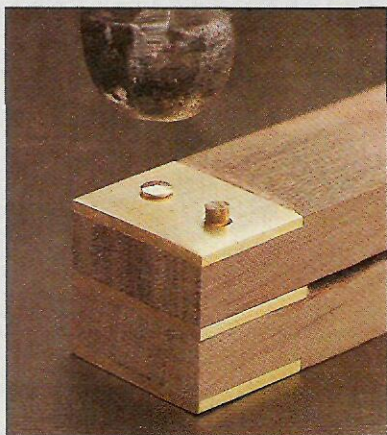
Rivets made from brass rod “draw” the handle pieces tightly together when the ends are peened over like a mushroom.
