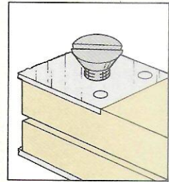
To align the top of the handle, insert a machine screw as a simple indexing pin.
