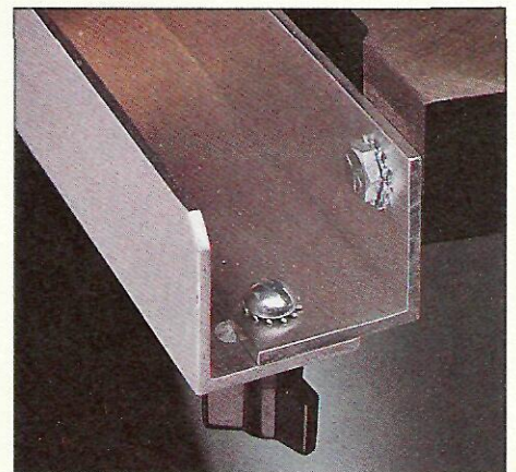
C. Adjustable Rail: The two-piece front rail is designed so you can adjust the angle of the fence to get a straight cut.
