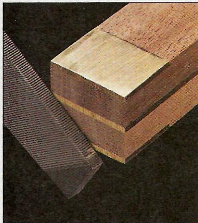
Shaping the ends of the handle is easy. You can use a smooth mill file (as shown), or a drum sander in a drill press.
