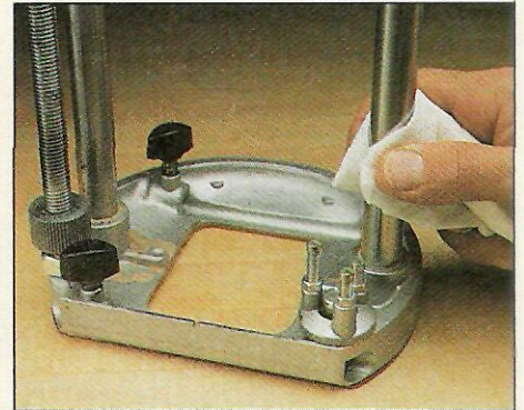
Plunge Tubes: Use a soft rag to clean the plunge tubes and rods. Then follow up the cleaning with a dry lubricant.
