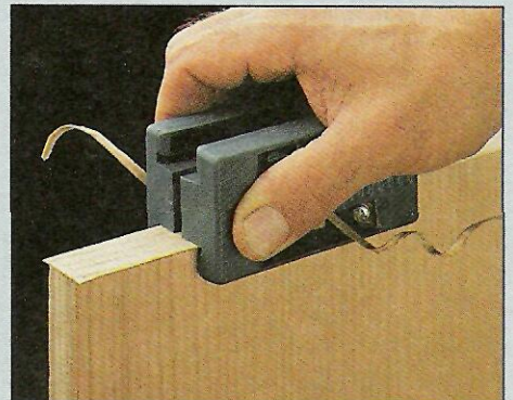
Double-Edge Trimmer. Spring-loaded sides on this trimmer adjust to the thickness of the plywood. Blades on each side remove both edges simultaneously.
