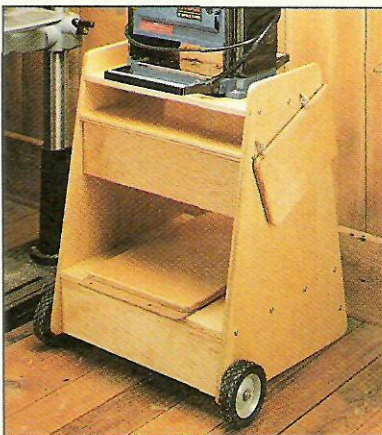
▲ The outfeed extension of the planer stand “knocks down” for moving and storage. The table lifts off and the “wings” fold back.
