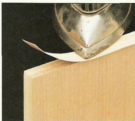
B. Iron-On Veneer. To glue this edging to the plywood, melt the layer of adhesive on the back with an ordinary iron.
