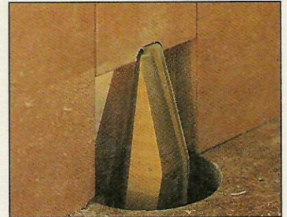
▲ To prevent chipout, a sliding insert forms a "zero-clearance" opening around the tip of the bit.
