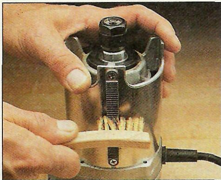
Rack and Pinion: I like to use a brass brush or an old toothbrush to clean the "teeth" on this type of height adjuster.
