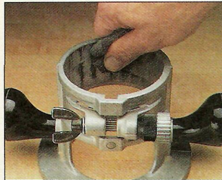
Pin and Groove: Steel wool works well to remove burrs and scratches that can form on the motor housing and base.
