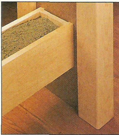
To add stability, a hollow wood beam is filled with sand. This anchors the stand and dampens the vibration of the lathe.
