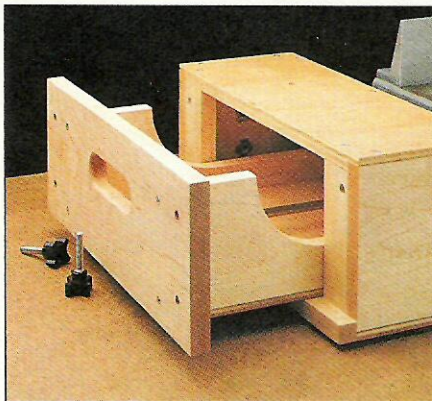
A. Wings: A pair of wings offer support to long stock and then "tuck" away inside the case for storage.
