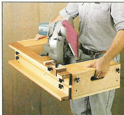
B. Portable: To make it easy to lift and carry the miter saw station, the wings have built-in handles.
