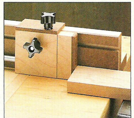
C. Stop System: For accurate repeat cuts, an adjustable stop slides in slots cut in the fence rails.
