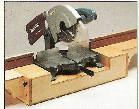
Miter Saw Station page 16
