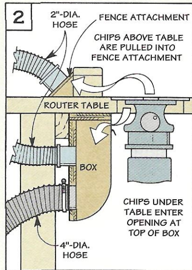
NOTE: TOP, BACK, AND SIDES CUT FROM 3/4"-THICK PLYWOOD
