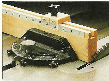
Miter Gauge Fence page 4
