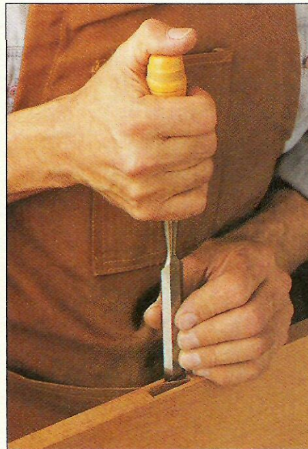
B. Overhand Grip. When making a vertical cut, an overhand grip lets you pare straight down. To help guide the blade, hold it loosely between your fingers.
