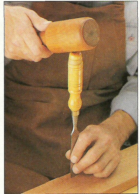
C. Blade Grip. Holding the blade of the chisel lets you pinpoint where the cutting edge enters the work. This is especially handy when using a mallet.
