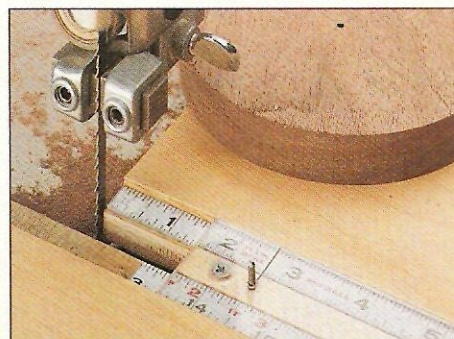
Band Saw Circle Jig page 4
