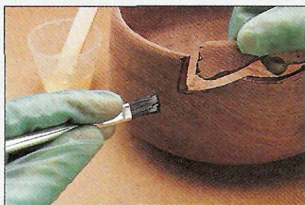
Step 1: Mix the resin and hardener together thoroughly and apply a coat to both surfaces to be joined.
