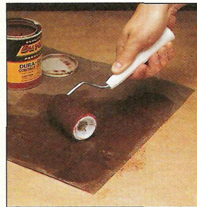
Step 2. Next, you can apply one or two coats of contact cement to the paper-backed side of the veneer.
