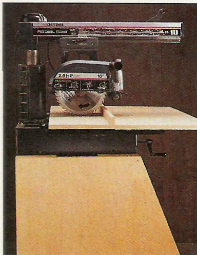
▲ If you have a saw with a short frame, you'll need to cut the sides at an angle to provide clearance for the height adjustment handle.
