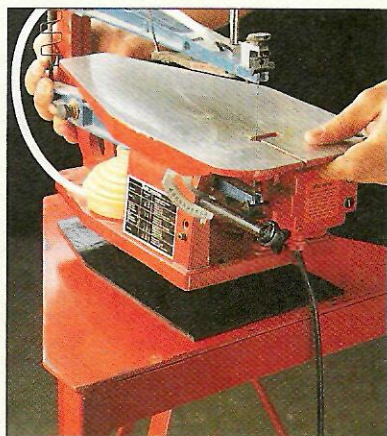
▲ Anti-Vibration Pad. This rubber-like pad absorbs vibration instead of transferring it to the stand.
