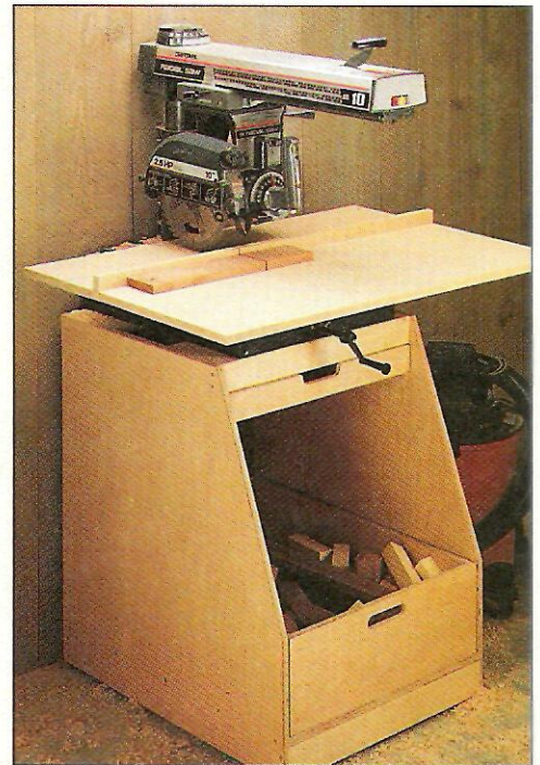
▲ The adaptable design of this radial arm saw stand allows you to build all or part of the storage system. You can just replace your old stand with a new base (photo above). Or build one or both lumber storage units (see front cover).
