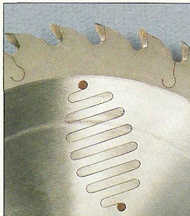
▲ Quiet Blade. Slots and sound-absorbing plugs reduce the noise level of this blade from 92 to 88 dB.
