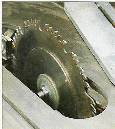
▲ Stabilizer. By adding side support, a stabilizer dampens noise produced by a wobbly blade.
