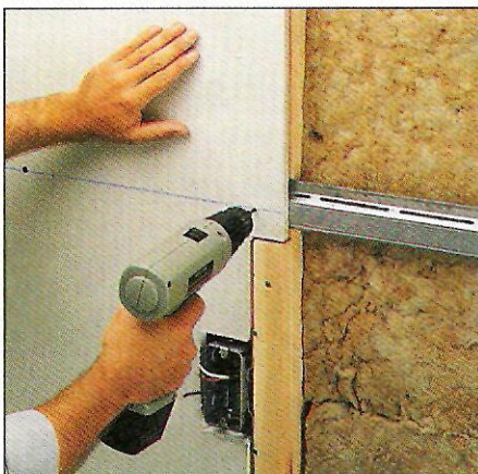
Step 4. Now you can screw a layer of drywall to the resilient channel. Use short screws so they don't hit the studs.
