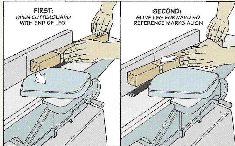
Step 4: With the leg against the fence, raise the end slightly above the table. Now nudge the cutter-guard open with the end of the leg and slide the workpiece forward until the reference marks align.
