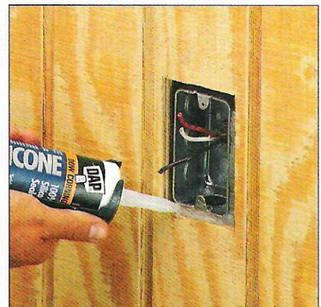
Step 6. To seal noise in, and still allow the walls to flex, fill in any gaps with a high-quality silicone caulk.
