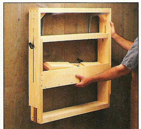
C. Compact Storage. When it’s not in use, you can knock down the sawhorse and store the feet in the tray.
