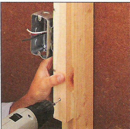
Step 1. Before you begin work on the ceiling or walls, you'll need to extend all of your electrical boxes.
