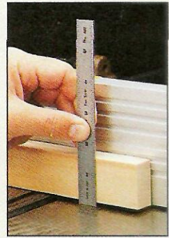
To determine the depth of cut, measure the gap between the infeed table and a straight stick laid across the outfeed table.
