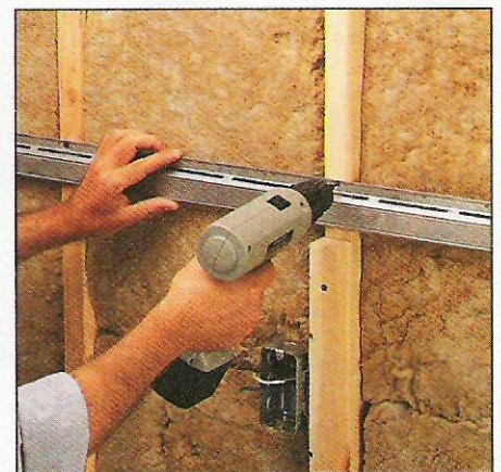
Step 3. With the sound blanket in place, screw lengths of resilient channel to the studs or joists.
