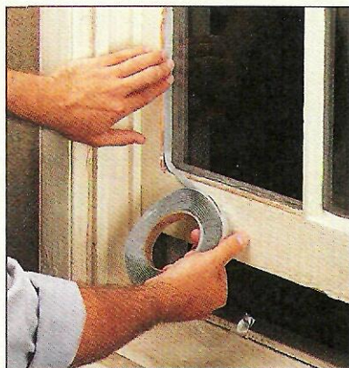
▲ Repair Windows. To seal windows for noise, first replace any broken glass and repair cracked or missing window glazing.
