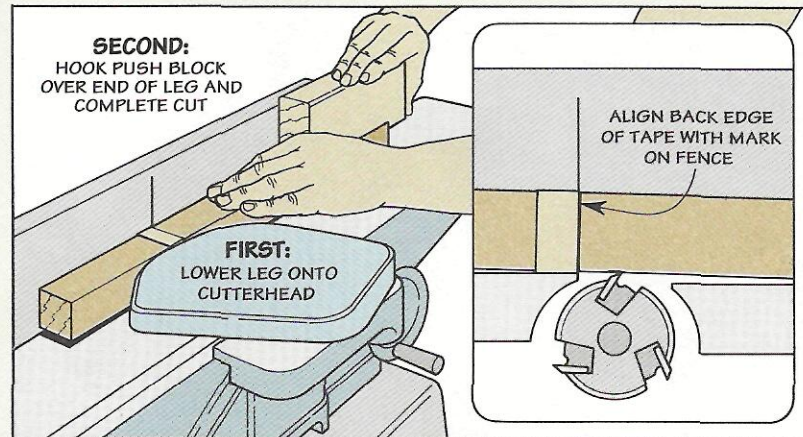
Step 5: When the back edge of the tape aligns with the mark on the fence, lower the leg down onto the cutterhead. Then hook a push block over the end of the leg and complete the cut.
