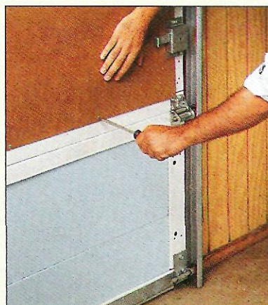
▲ Overhead Doors. You can increase the STC of a garage door by filling the panels with insulation and covering it with Masonite.
