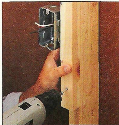
▲ Stud Extension. Extend electrical fixtures so they're flush with your new wall by widening studs with scrap "two-by" material.
