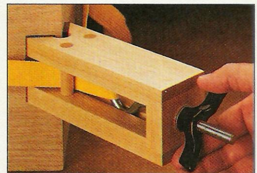
▲ Now fit the jaws of the clamp on a corner of the project, reposition the strap (if necessary), and tighten the wing nut.
