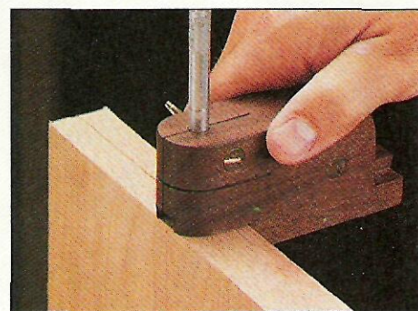
C. Cutting Gauge. Using the leftover material, you can make a second head to hold an X-Acto knife. This will allow you to score layout lines.
