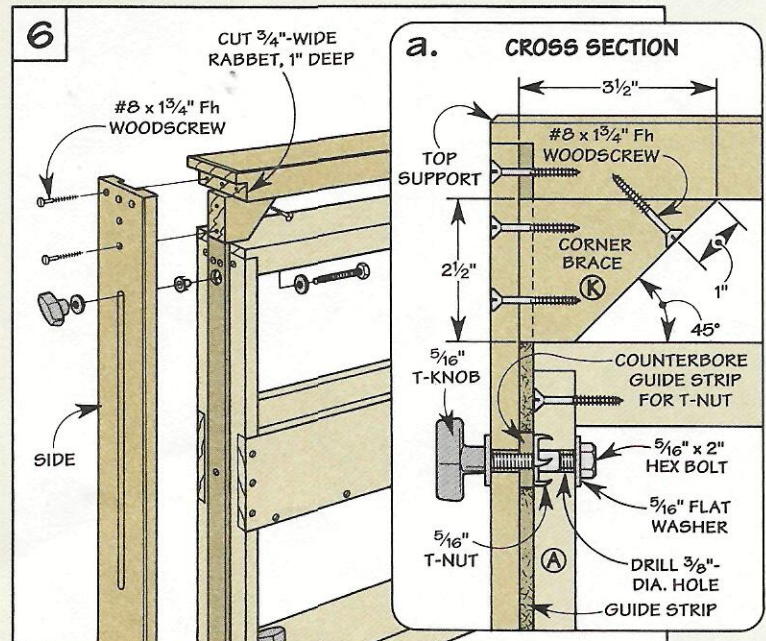
With the support pushed all the way down, use a brad point drill bit to locate the hole for each hex bolt.
