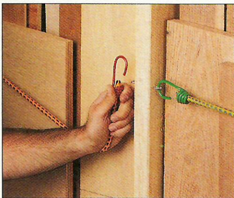
▲ To hold "shorts" in place, I installed screw eyes in the uprights and ran stretch cords across the storage compartments.
