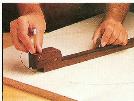
B. Beam Compass. When used as a beam compass, the layout tool allows you to lay out just about any size arc or circle you'll need.
