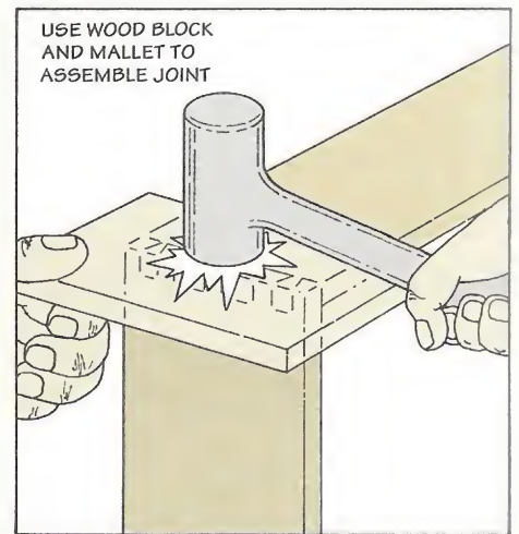
Step 6. After applying a small amount of glue to the leading edges of the pins, use a wood block and a mallet to drive the joint together.
