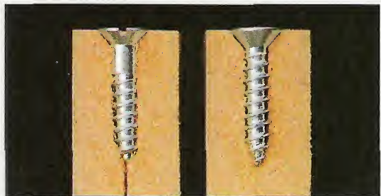
▲ It's possible to split MDF when drilling and screwing into the edge with a tapered wood-screw, left. To avoid this, drill a pilot hole and use a straight-shanked screw, right.
