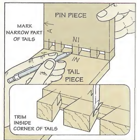
Step 3. Next, check that the wide part of the pins fits the openings on the inside face of the tail piece. Then mark the tails and trim as before.
