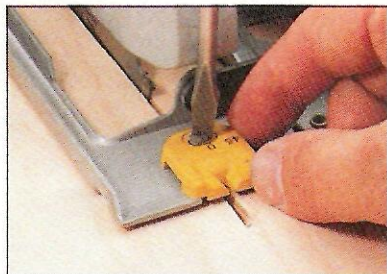
tor on the Quantum (right) can be adjusted if you use blades that vary in thickness.
