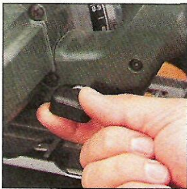
Depth Adjustment. The plastic knob on the Quantum (left) provides a more comfortable grip than the wing nut on the B&D (center). But neither are knuckle-busters like the depth adjustment lever on the Skil (right).
