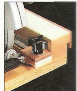
Depending on your saw, you may need to modify the front or back brackets.
