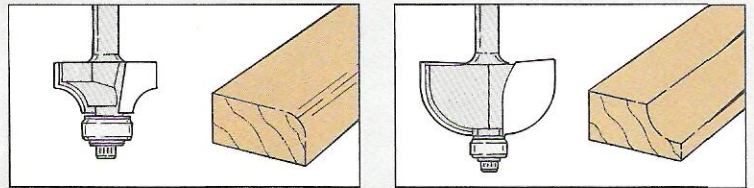
Round-Over. Round-overs come in many sizes. They look best on the top of a molding.
