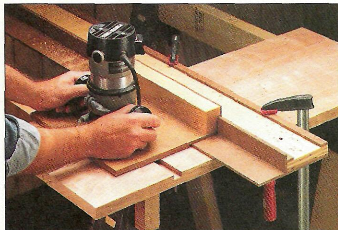
Router. With the cutting guide clamped across a wide panel, it can also be used to turn your hand-held router into a precision tool when routing dados (or grooves).
