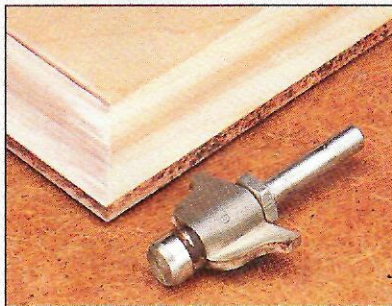
▲ Solid Pilot. As a solid pilot rubs against the edge of the workpiece during a cut, it tends to burn or burnish the surface.
