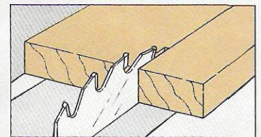
Straight Cut. One of the simplest ways to top off a profile is to add a straight-ripped edge.
