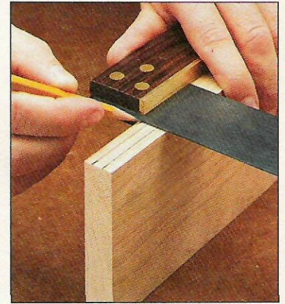
Length. Use a try square to lay out the shoulders and determine the length of the tenon.
