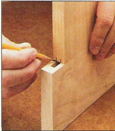
Thickness. To establish the thickness of the tenon, draw lines just inside the walls of the mortise.
