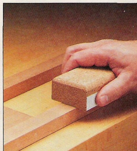
C. Hand Sanding. But on a narrow workpiece, a sanding block ensures a crisp corner and a flat surface.
