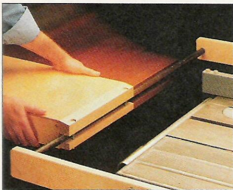
A. Position. You can position the outfeed table anywhere across the back of the table saw — for any size workpiece.
