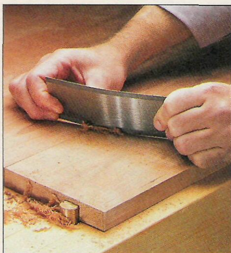
A. Scraper. Use a scraper to remove any tool marks or ridges. Skew the scraper at an angle for the best cut.
