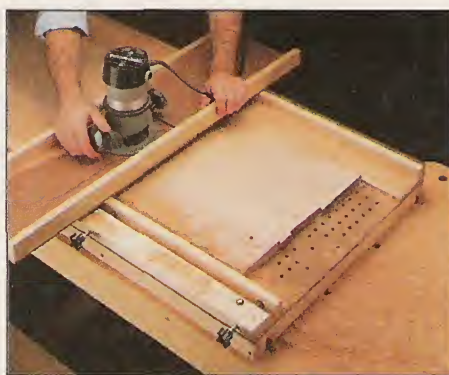
B. Wide Panels. The thicknessing jig can handle glued-up panels and wide boards up to 15 3/4" in width.
