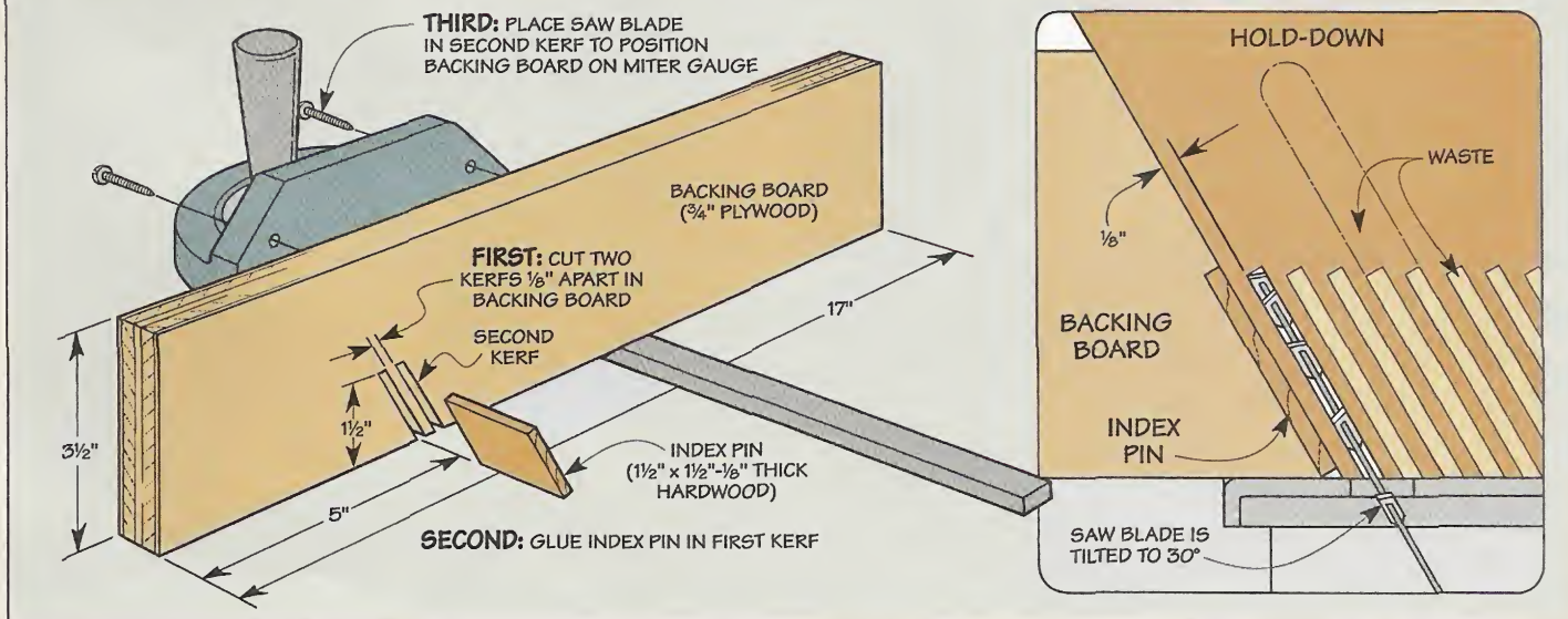
Perfect Kerfs. The index pin makes it easy to cut evenly-spaced kerfs. Just index the workpiece on the pin between each pass.
