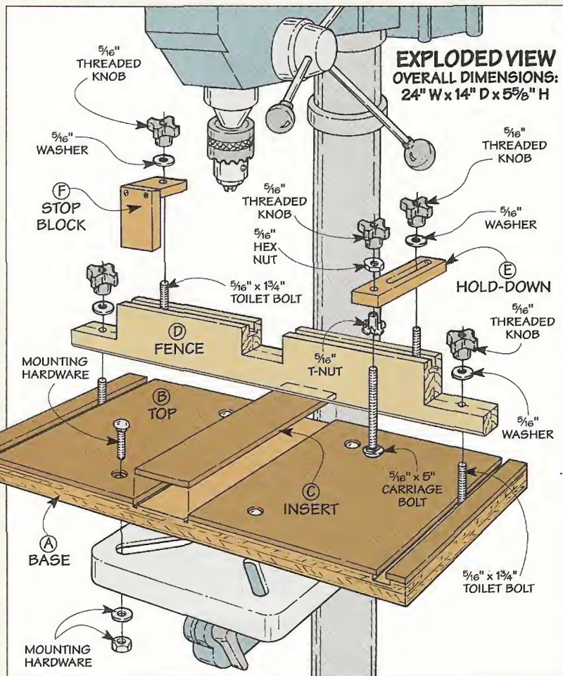
Accurate Drilling. The fence on this drill press table uses a stop block and a hold-down for clamping and accurately positioning a workpiece.
