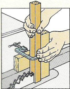
A safe way to cut an open mortise on a long workpiece is to clamp it to a support jig that's made by screwing scraps of 2x4 together.
