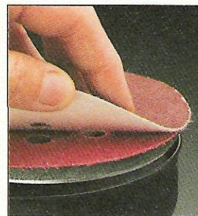
Pads. A hook & loop system (left) makes it quicker and easier to change sanding discs than a pad that uses pressure sensitive adhesive discs (right).
