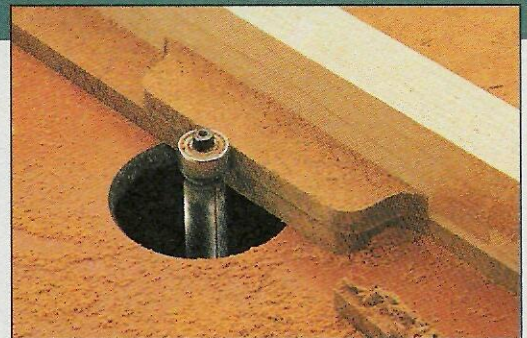
Identical Parts. A quick way to produce identical parts is to make a template and use it as a pattern for a flush trim bit to follow.
