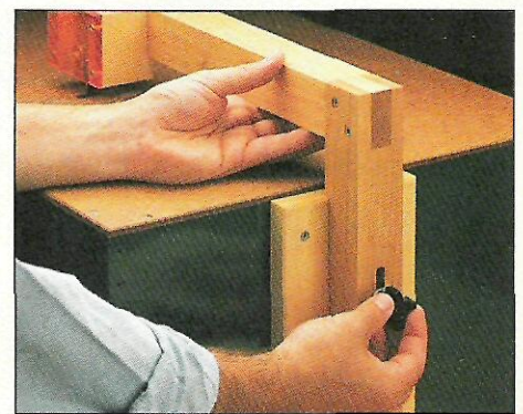
C. Adjustable Arm. The arm that supports the guide system and hold-down adjusts for different thicknesses of stock.
