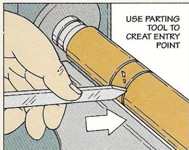
Step 1. After laying out the cove, push the tip of a parting tool into the work to make a shallow V-cut.
