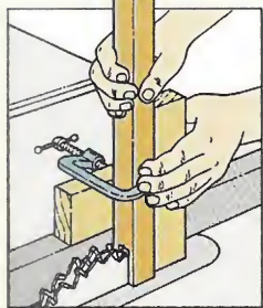
A safe way to cut an open mortise on a long workpiece is to clamp it to a support jig that's made by screwing scraps of 2x4 together.
