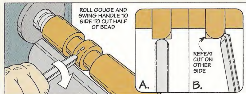
Step 2. Start with the gouge on its back and the handle well down. Then raise the handle and
