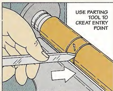
Step 1. After laying out the cove, push the tip of a parting tool into the work to make a shallow V-cut.
