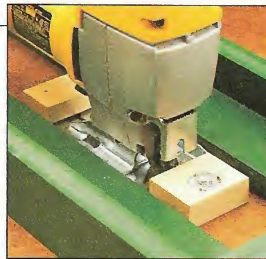
▲ In addition to cleats that keep the saw from moving side to side, two wood blocks lock it in place.
