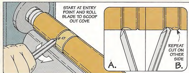
Step 2. With the flute on the gouge facing the intended cove, push the tip firmly into the V-cut (left).
