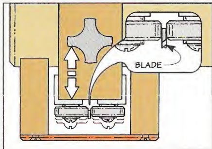
Step 1. Slide the adjustment block forward (or back) so the bearings are right behind the teeth on the saw.
