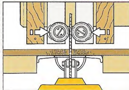
Step 2. Now remove the guard and position the bearings close to (but not touching) the saw blade.
