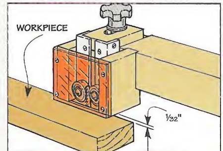
Step 3. Finally, adjust the arm so the hold-down is about \frac{1}{32} " above the workpiece and lock it in place.
