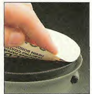
Pads. A hook & loop system (left) makes it quicker and easier to change sanding discs than a pad that uses pressure sensitive adhesive discs (right).
