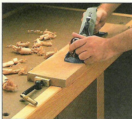
B. Bench Dog. A hex bolt (photo A) and a Veritas Wonder Dog make a functional bench dog system.
