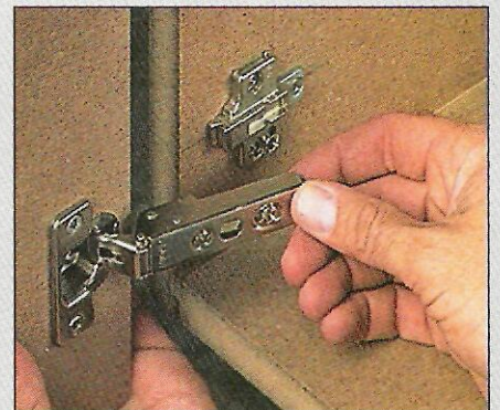
Step 3. To hang a door, just snap the hinge clip on the mounting plate, then adjust the hinges to position the door.
