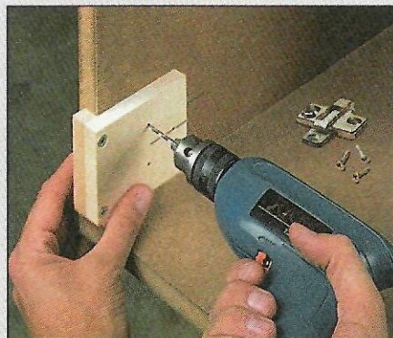
Step 2. Next, drill pilot holes in the side of the cabinet for the mounting plate screws, refer to template above.
