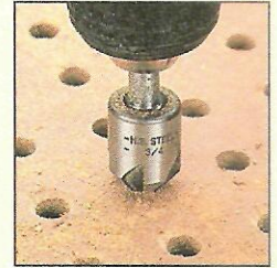
To increase airflow, first enlarge the holes in the top. Then chamfer the edges with a countersink.
