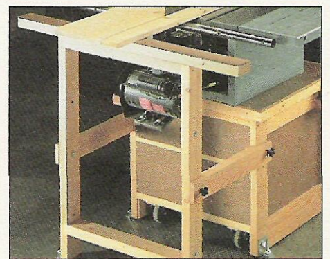
C. Outfeed. To make cutting large workpieces more manageable, an outfeed support attaches to the stand.
