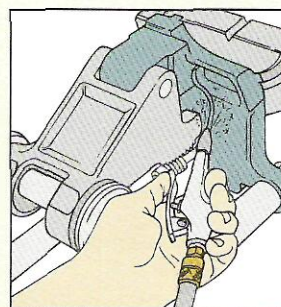
Clean Saw. To clean a table saw, the first step is to blow away any trapped sawdust from inside the saw cabinet. Then scrub away the pitch and resin build-up.
