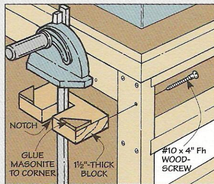
Miter Gauge. A block with a notch cut in it holds the miter gauge. And scraps of Masonite keep it from slipping off.
