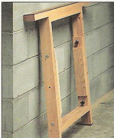
▲ Storage. For compact storage, tuck the arms that connect the outfeed support to the cabinet inside the frame and tighten the knobs.
