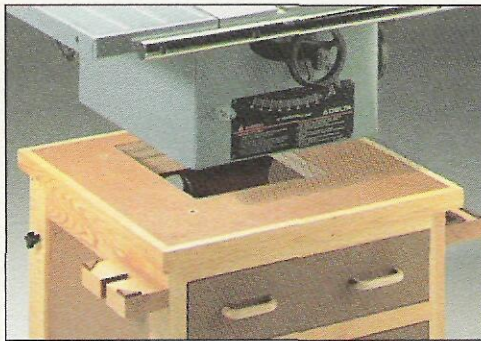
▲ A built-up top with a hole cut in it allows sawdust to fall through. It also provides a sturdy platform to mount the table saw.
