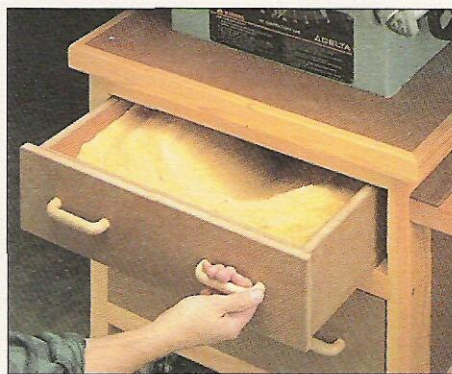
B. Dust Bin. A bin below the saw cabinet collects dust. When it’s full, the bin pulls out for easy emptying.
