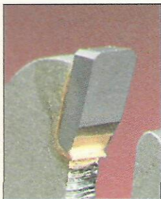
Chamfers on the raker teeth of the CMT blade help prevent chipout.
