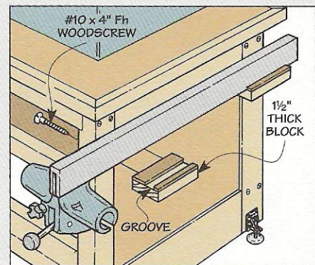
Rip Fence. To hold the rip fence, these brackets have grooves formed by gluing strips of Masonite to a wood block.
