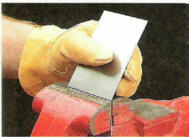
Cutting a Scraper. After filing a deep groove across the blade (top), tighten the scraper in a vise and bend it until it snaps (bottom).
