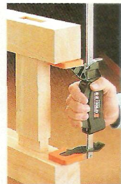
Simply reversing the jaws on the E-Z Hold clamp allows you to use it as a spreader.
