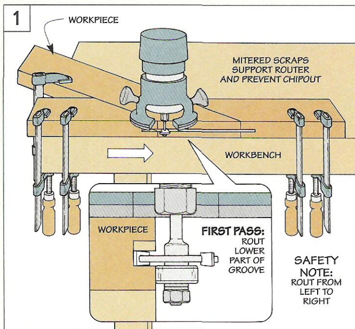
A slot cutter bit makes quick work of routing a groove for a spline. And different size bearings let you adjust the depth of cut.
