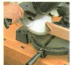
With the head tilted to 45°, cut a tall scrap piece that's standing on edge.
