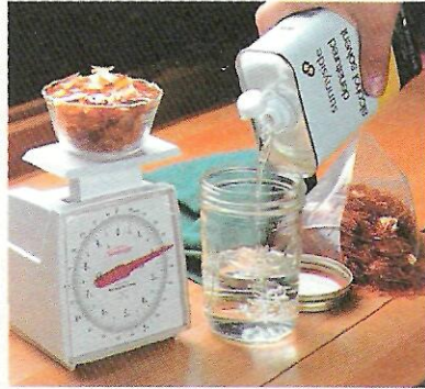
A. Cut. Weigh the flakes of shellac and measure out the alcohol to determine the correct "cut."
