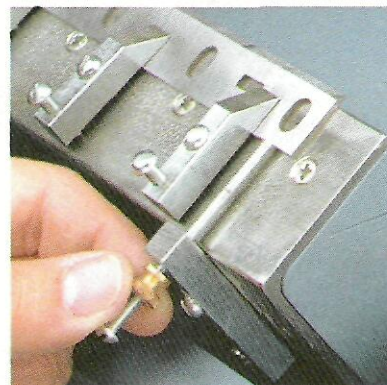
A. Stop. A micro-adjustable stop lets you fine tune the position of the knife. And a set of hold-downs keeps it securely in place.
