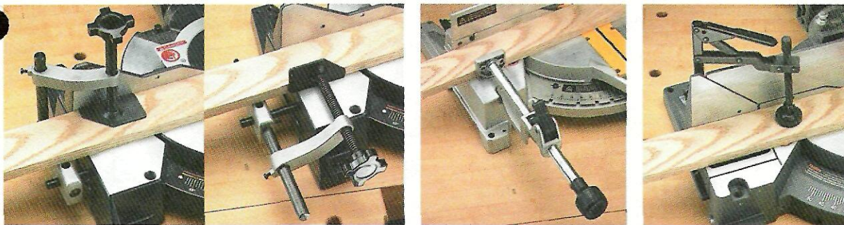
Hold-Downs. The hold-down on the Sears can be used to clamp work down against the saw table (left) or against the fence (left center). So it has a wider range of uses than the DeWalt (right center) that holds work against the fence only, or the Skil (right) that only applies pressure downward.
