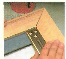
Now form a "corner" with the two cutoffs and check it for square.
