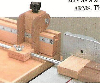
To cut short pieces, an auxiliary stop extends over the metal saw table. It's just a wood block that's held onto the end of a metal rod with epoxy.
