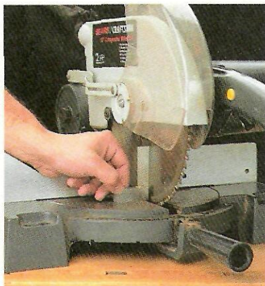
A. Set 0° Stop. After adjusting the 0° stop so it contacts a casting on the arm, align the indicator to the 0° mark on the bevel scale.
