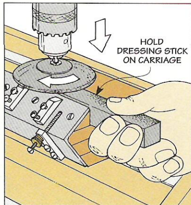
Step 3. Lower the spinning grinding stone onto a dressing stick to "true up" the stone.
