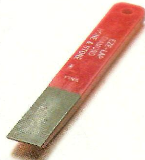
Use a fine diamond hone to remove the burr and add a secondary bevel to the edge of the knife.
