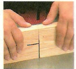
Now flip one of the cutoffs over and butt the pieces end to end to see if there's a gap.
