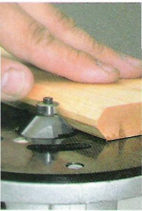
Chamfer Gauge. A scrap block with pre-cut chamfers makes it easy to set the height of the chamfer bit.
