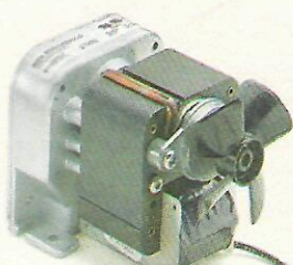
The heart of the oscillating drum sander is a small, electric gearmotor.
