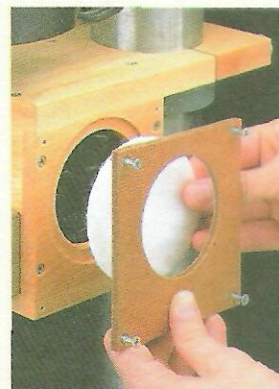
The back of the motor housing encloses an ordinary filter from a dust mask.
