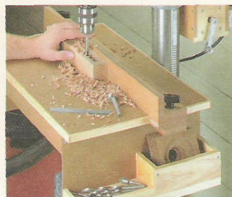
C. Fence. A simple fence with a built-in clamping system also lets you use the sanding platform as a drill press table.
