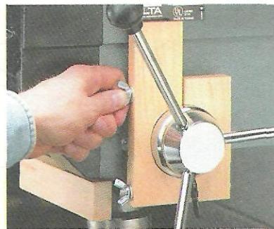
Step 3. Position the pinch block straight up and down and tighten it around the hub of the feed lever.
