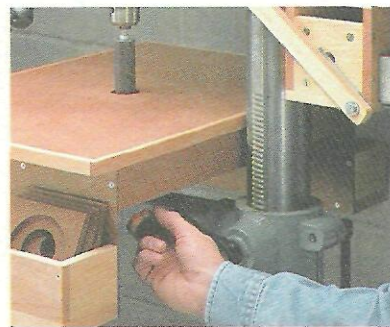
Step 6. Finally, remove the scrap block (see Step 2) and adjust the height of the sanding platform.
