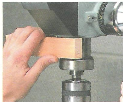
Step 2. Before attaching the arm, use a 1½" tall (wide) block to temporarily hold the quill down.
