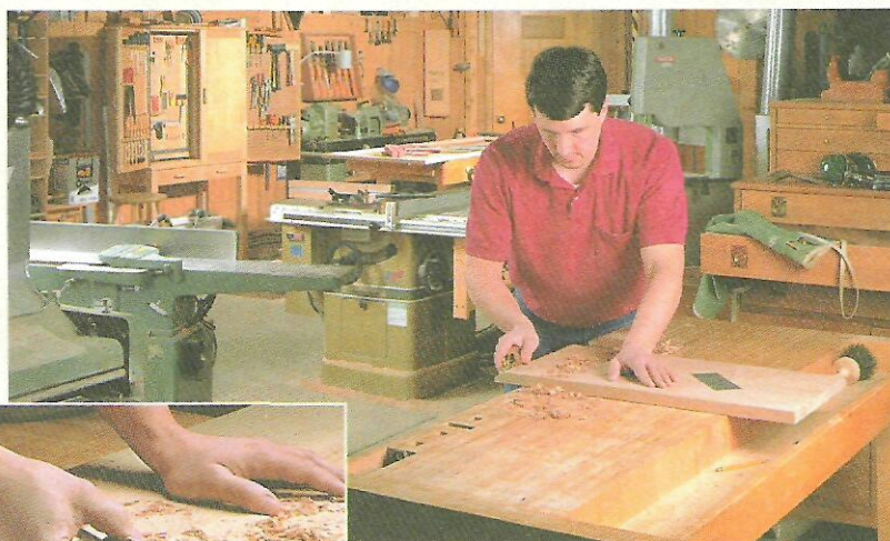
▲ Steve Johnson (our shop craftsman) chamfers the end of a glued-up panel with his Lie-Nielsen low-angle block plane.
