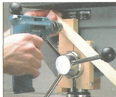
Step 5. After drilling a hole in the top end of the arm, cut it to length and attach it to the pinch block.
