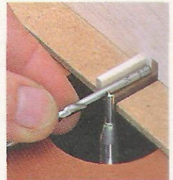
An \frac{1}{8} " drill bit makes a handy gauge to help position the key.
