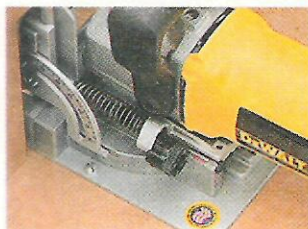
Holes in the base of this DeWalt joiner can be used to screw it directly in place.
