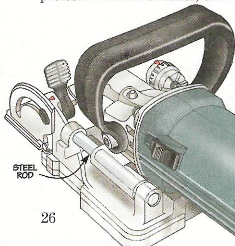
BODY OF PLATE JOINER SLIDES ON MACHINED STEEL RODS
