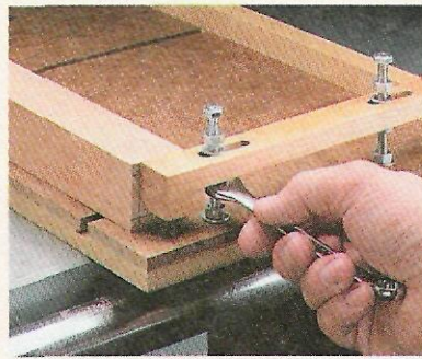
Step 2. With the leg in place, adjust the hex nuts up or down so it sits flat on the platform.
