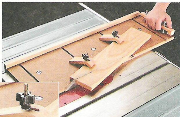
Angled Cuts. Two adjustable hold-downs clamp work securely in place when making angled cuts.
