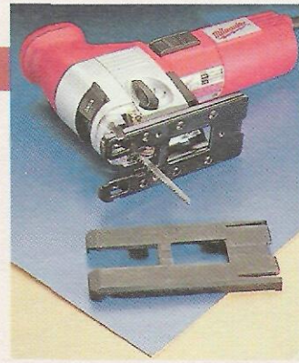
◀ Snap-on Base Plate. To protect surfaces that get scratched easily, the Milwaukee and DeWalt have a plastic base plate that snaps quickly onto the metal base of the saw.
