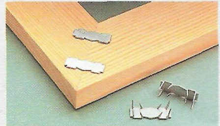
Tack Plates. The sharp, angled claws on the bottom of these metal tack plates help reinforce the miter joint.
