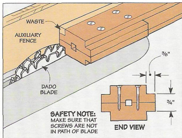
3 Cutting a rabbet on all four edges of the clamp head forms a tongue on each side that will guide it in and out of the miter trimmer.
