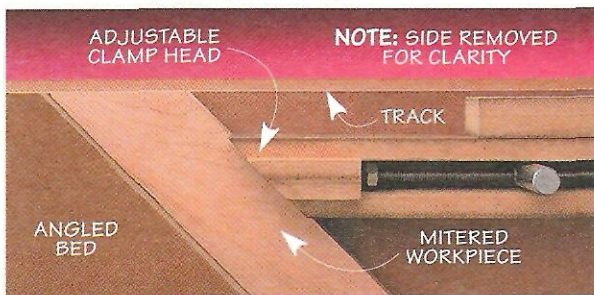
A. Position Workpiece. With the mitered end of the workpiece flush with a track in the top edge, a clamp head presses it against an angled bed.
