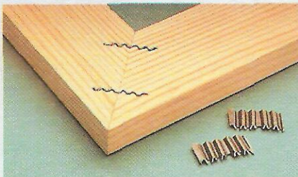
Corrugated Nails. The ridges on these corrugated nails hold the mitered corner of the frame tightly together.
