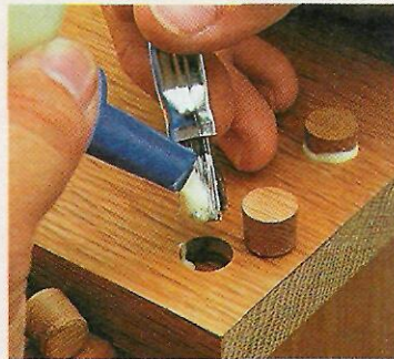
4 After brushing glue around the sides of the hole, tap the plug in place so it's snug.
