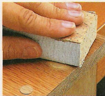
6 Finally, sand each of the plugs flush with the surface of the workpiece.
