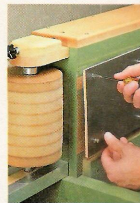
▲ To make the platen easy to replace if it gets worn, it's simply screwed to the sleeve.
