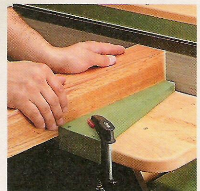
▲ Stop. Clamping a stop to the front table allows you to sand the ends of a workpiece square.
