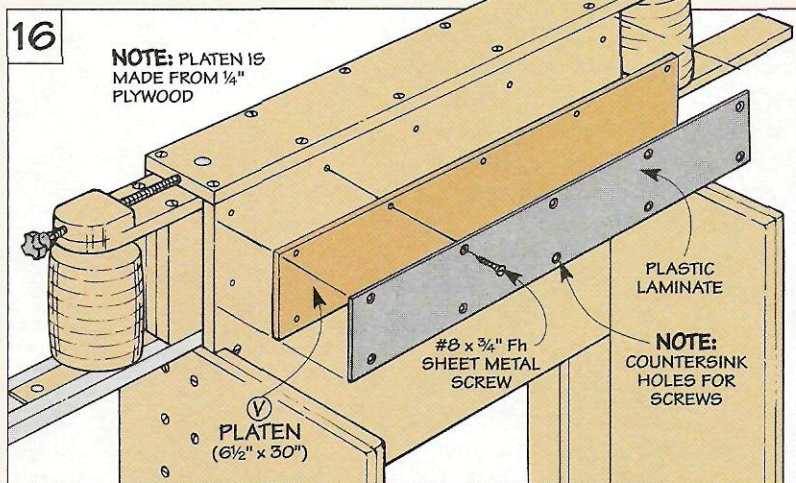
▲ To make the platen easy to replace if it gets worn, it's simply screwed to the sleeve.
