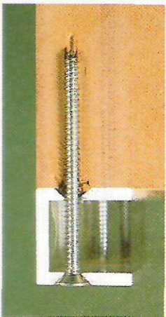
▲ A countersink on the bottom of the aluminum channel recesses the screw head. The one on top forms a pocket for any wood fibers that pull out as you drive in the screw.
