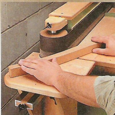
▲ Curved Pieces. An end table "wraps" around a roller so you can sand curved workpieces.
