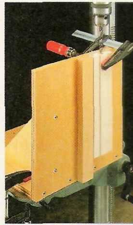
▲ An L-shaped support with a vertical cleat makes it easy to drill a hole in the end of a long workpiece like the adjustment block.
