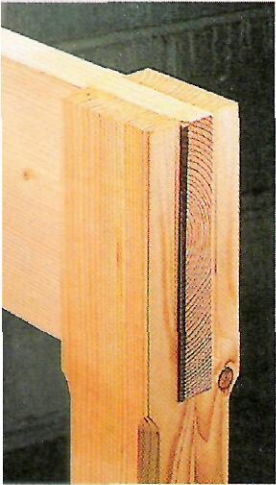
▲ A strong mortise and through tenon joint provides the cornerstone for a sturdy base.
