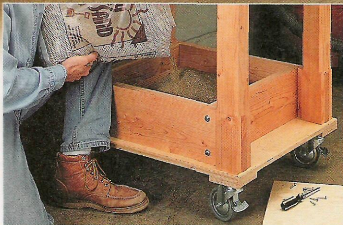
A. Sandbox. To add stability, a "sandbox" in the bottom of the stand holds about 100 lbs. of sand. This extra ballast prevents the stand from tipping when you roll it around.
