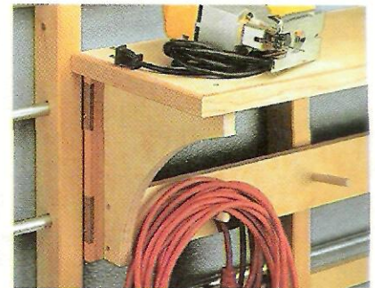
▲ To provide storage under the shelf, glue dowels into angled holes drilled in the stretcher.
