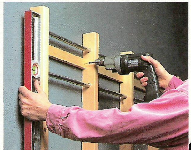
2 After checking that the uprights are level and plumb, attach the grid by driving screws through the cleats and into the wall studs.
