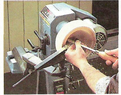
▲ Outboard Turning. The headstocks on all these lathes can be rotated 90° to the bed (left). This lets you turn large diameter workpieces. And it positions the workpiece for easy access (right).
