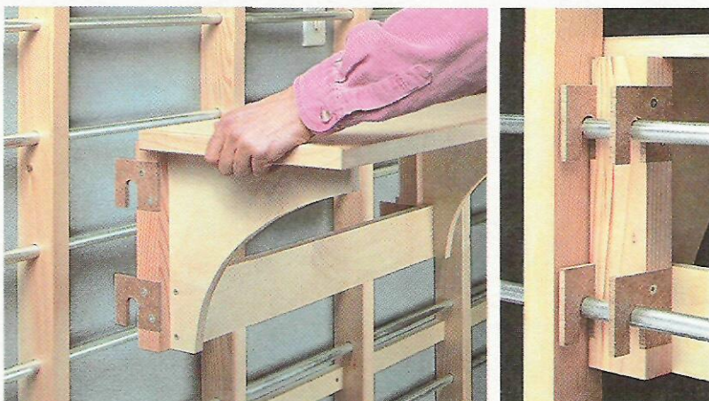
▲ It's easy to hang each storage unit exactly where you want on the grid (left). The secret is a set of hanging brackets attached to the back of each unit that fit securely over the metal conduit (right).
