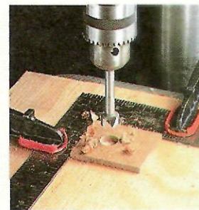
▲ A framing square clamped to the drill press table makes it easy to position the hooks quickly and accurately when drilling holes for the slots.
