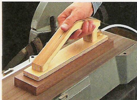
▲ Push Block. This push block works together with the vacuum system to provide a firm grip on a workpiece.
