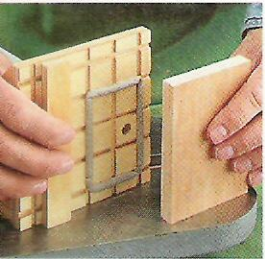
▲ An alignment strip lets you position a workpiece quickly and accurately on the vacuum plate. After applying the vacuum, just set the strip aside.
