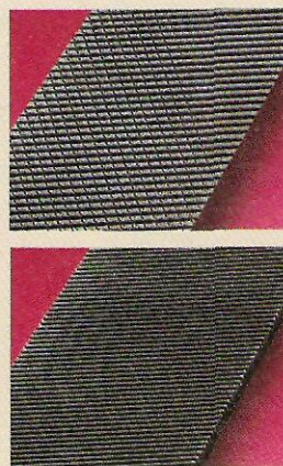
The diamond-shaped cutting edges on a double-cut file (top) remove material more aggressively than a single-cut file (bottom).
