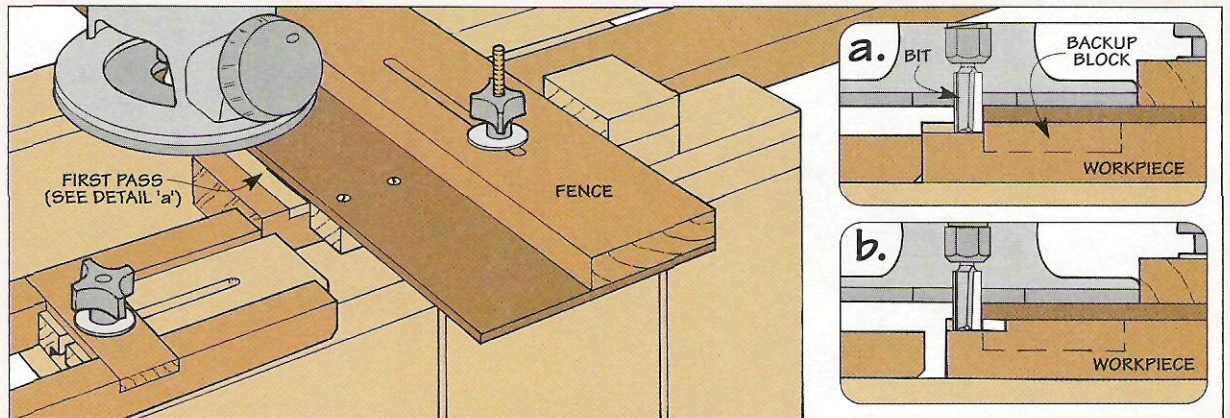
3 With the base of the router riding against the fence, cut the shoulder of the cheek first, see detail 'a.' If you need to make additional passes to
