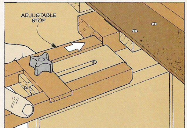
2 Now slide the adjustable stop against the end of the workpiece and lock it in place. The stop ensures that all four shoulders align.
