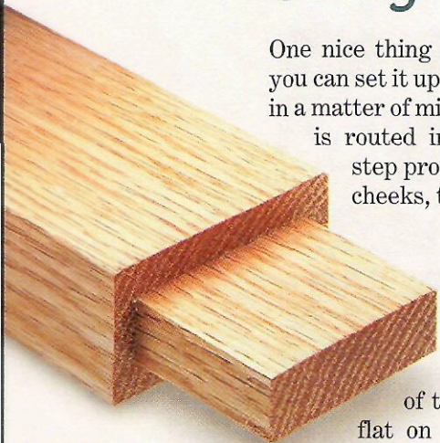
▲ It only takes a few minutes to set up the jig and rout a straight, square-shouldered tenon.
