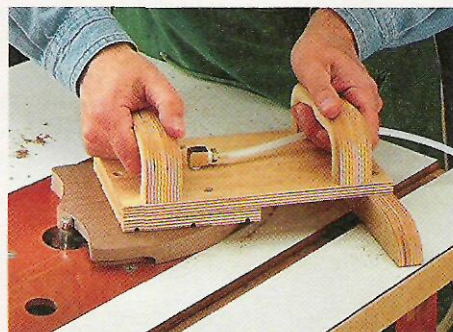
▲ Routing Jig. A vacuum allows this jig to hold small parts so you can rout them safely on a router table.
