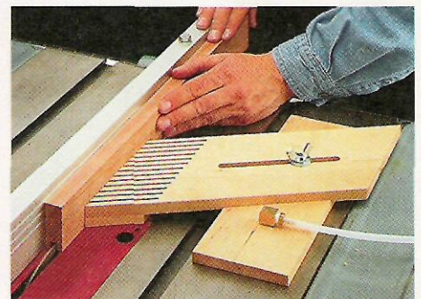
▲ Featherboard. All it takes to attach this featherboard to a table saw is to flip a switch on the vacuum system.
