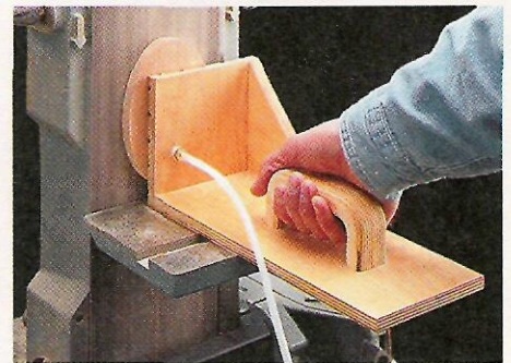
▶ Small-Piece Sanding Jig. A vacuum plate in the front of this jig makes it easy to sand small workpieces safely.
