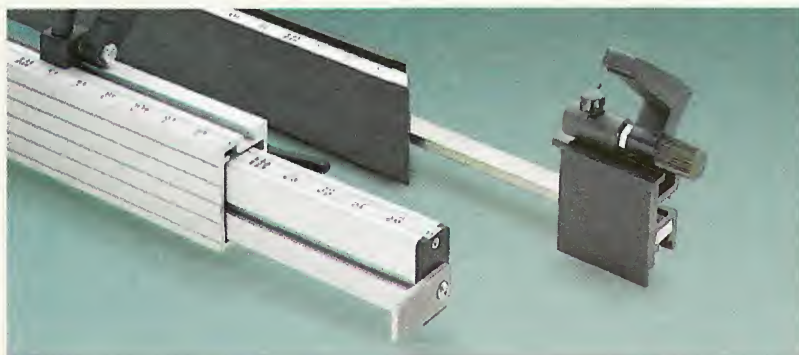
Fence Extensions. To cut long pieces to length, the flip stop on the Vega attaches to an extension that slides out of the fence (right). The Accu-Miter (left) has an extension with a stop attached to the end.
