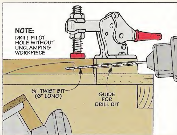
3 There's no need to unclamp the workpiece to drill the pilot hole. The guide in the fence will automatically center the twist bit on the pocket.
