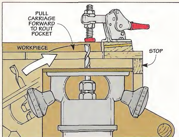
2 After turning the router on, slowly pull the carriage forward until it stops. As the carriage pivots, the router bit scoops out the pocket in the workpiece.
