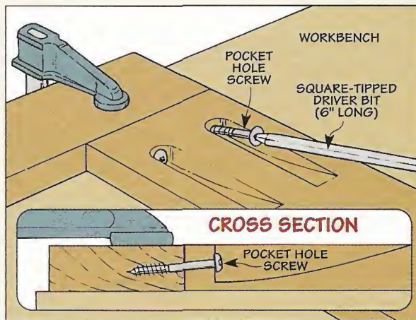
4 To assemble the joint, place both workpieces on a flat surface. Then clamp the back piece in place and use a long driver bit to install the screws.
