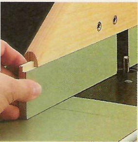
▲ To quickly adjust the fence opening for different size bits, just move the sliding faces in or out as needed.
