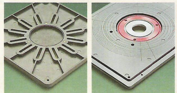
▲ Mounting Systems. Slots in a plate (left) act as a universal mounting system for a router. But the rings (right) make it easier to center the bit in the opening.
