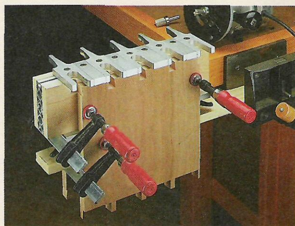
B. Katie Jig. Sometimes simple is best. This Katie Jig allows you to rout through-dovetail joints quickly and accurately without the usual trial and error process.
