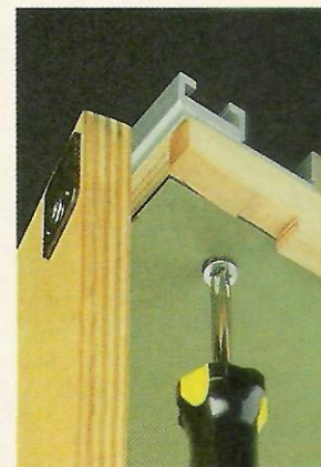
▲ An adjustment screw lets you "tweak" the wings to create a flat, level worksurface.
