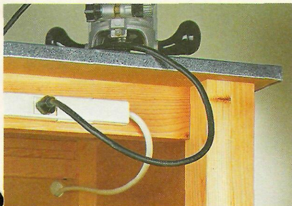
▲ Power Strip. To provide a convenient plug-in for my portable tools, I attached a power strip to the bench. The power cord for the strip feeds out a hole in back.
