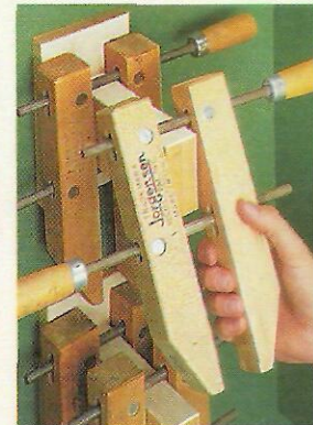
▲ All it takes to hold handscrews is a simple wood block.
