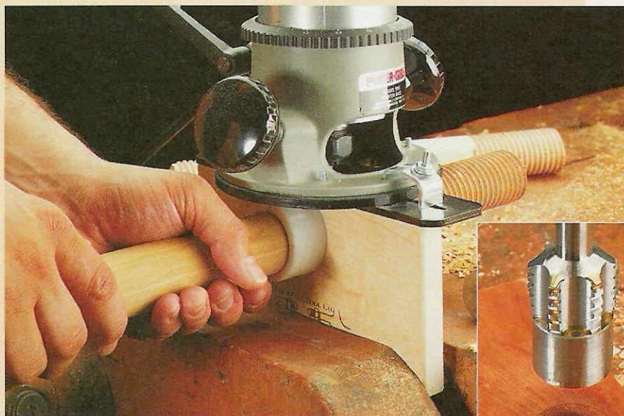
▲ To rout the outside threads in a dowel, twist it through the plastic insert in this jig like you're making sausage. A hand-held tap cuts the inside threads, see inset photo.
