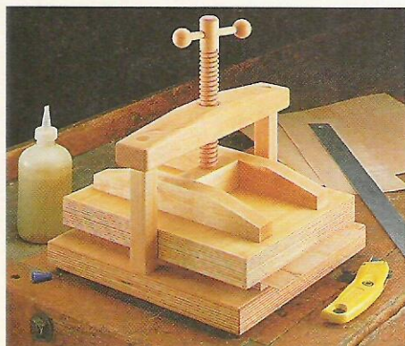
▲ Veneer Press. Tightening a single wood screw applies all the clamping pressure that's needed for this small veneer press.
