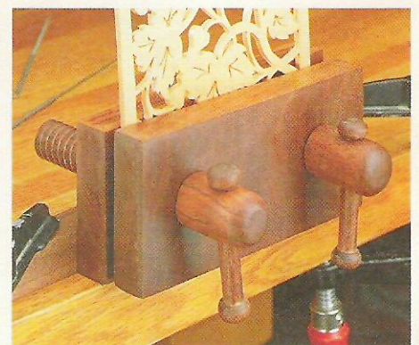
▲ Benchtop Vise. The twin wood screws on this small, benchtop vise thread into tapped holes in the back jaw.
