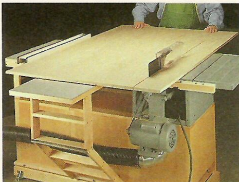
A. Rip Fence. Adding a precision rip fence and a large extension table makes it easy to rip sheet material up to 40" wide.
