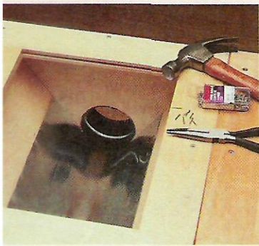
▲ An angled trough covered with a thin sheet of metal directs chips out the opening in back of the cabinet and into a dust collector.
