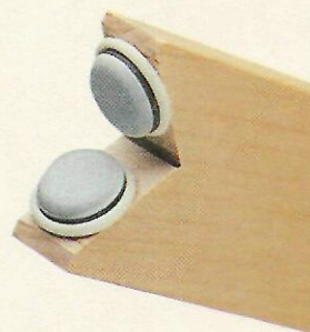
▲ Adding two nylon furniture glides to the notched end of each leg allows the lower support to slide smoothly on the lower rail.
