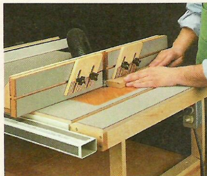
B. Router Table. To save space, the extension table doubles as a router table. There's even a removable fence.
