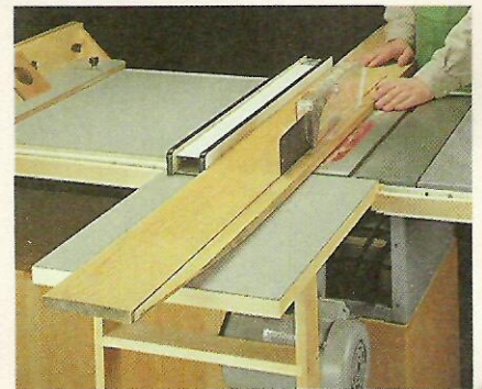
C. Outfeed Support. A simple outfeed table provides plenty of support when ripping a long workpiece.
