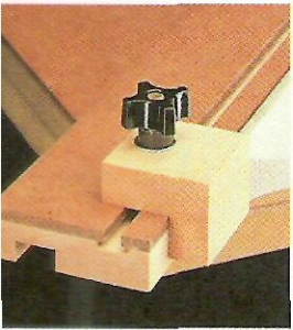
▲ Stop Block. An adjustable stop block provides a quick, accurate way to miter pieces to identical lengths.
