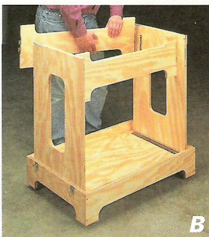
Setup. It only takes a minute to set up the workbench. After unlatching the top and setting it aside, remove the stretchers and flip up the sides, as shown in photo 'A.' To provide rigid
