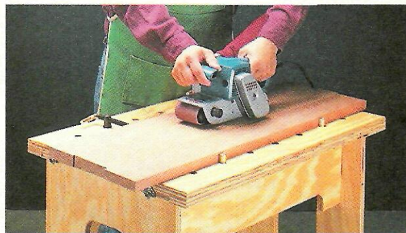
◀ Bench Dogs. Using one (or more) pairs of bench dogs lets you hold work tightly against the top without clamps getting in the way.
