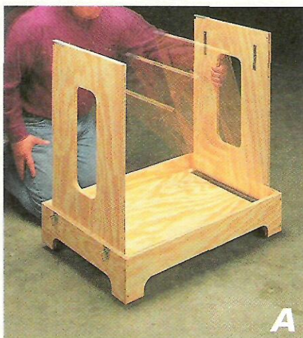
Setup. It only takes a minute to set up the workbench. After unlatching the top and setting it aside, remove the stretchers and flip up the sides, as shown in photo 'A.' To provide rigid
