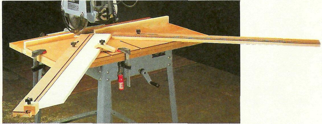
▲ Long Fences. As an option, you may want to build a pair of 48"-long fences to use when mitering extra-long workpieces. With the stop block set at the end of the fence, you can cut pieces up to 46" long.
