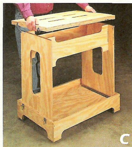
support for the top of the bench, the stretchers hook into the sides (Photo B). Then just fit the top down over the sides of the bench and pull it toward you to “lock” it in place (Photo C).
