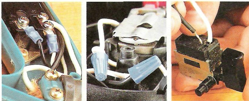
▲ Connectors. The wires from the power cord may be attached with crimp-on connectors (left), wire nuts (center), or a spring-loaded mechanism in the switch (right). Just be sure they're tight so they don't wiggle loose.
