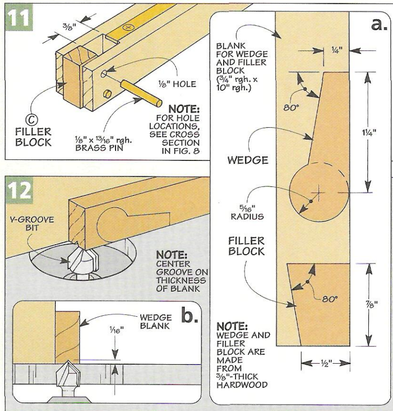
▲ To fit the wedge into the opening in the beam, sand the sides lightly on a flat surface.
