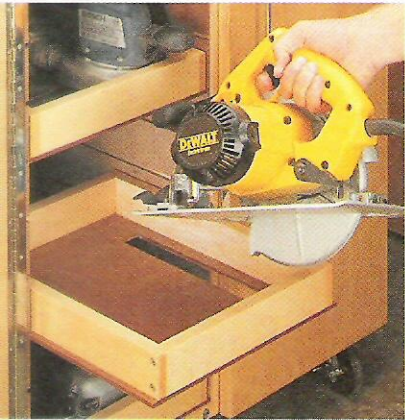
▲ To allow my circular saw to sit flat, I cut a long slot in the bottom of the tray that's wide enough to fit the blade guard.
