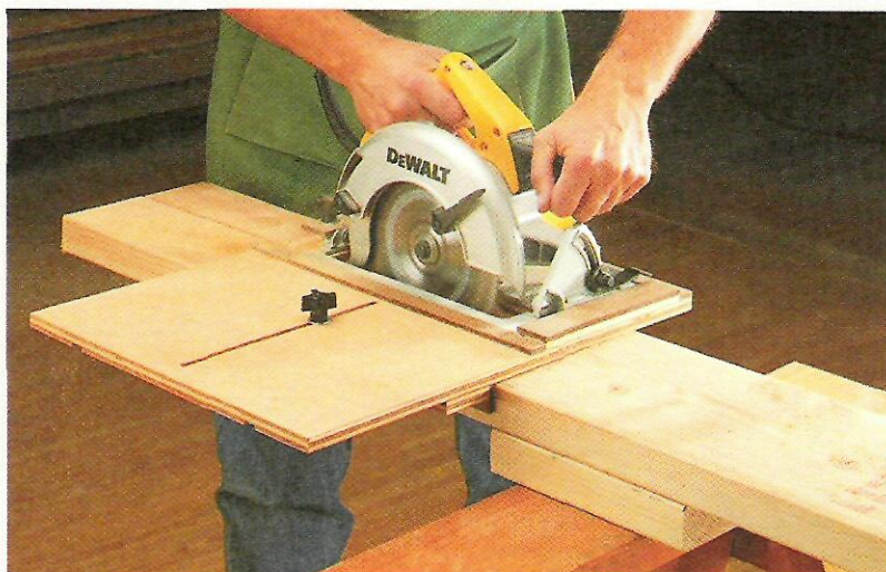
Edge Guide ▶ Plow perfectly straight rip cuts with this adjustable edge guide. Notice the block underneath that prevents the blade from cutting into the sawhorse.
