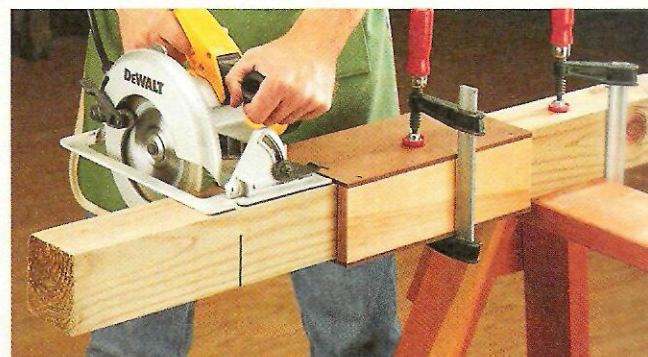
▲ Cutoff Saddle. To ensure smooth, square cuts when working with thick lumber, this cutoff saddle guides the saw when making cuts from two opposite sides of the post.
