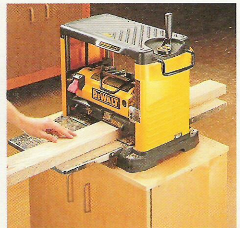
C. Tool Stand. With a sturdy top and a set of locking casters, this cart can also serve as a stable platform for a benchtop tool.
