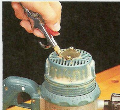
A. Remove Dust – With the tool running, blow air through the intake slots to remove packed-in dust.
