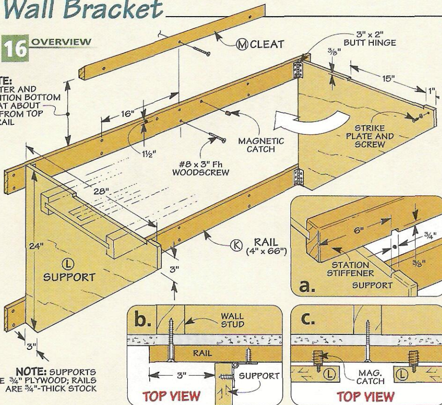
▲ After removing the miter saw, storing the station is just a matter of hanging it on a cleat and folding the supports for the station against the wall.
