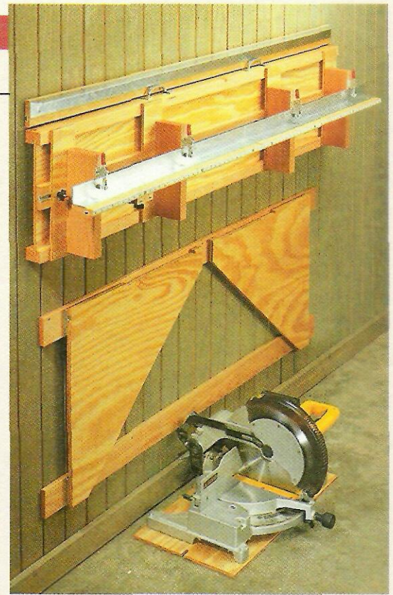
▲ After removing the miter saw, storing the station is just a matter of hanging it on a cleat and folding the supports for the station against the wall.
