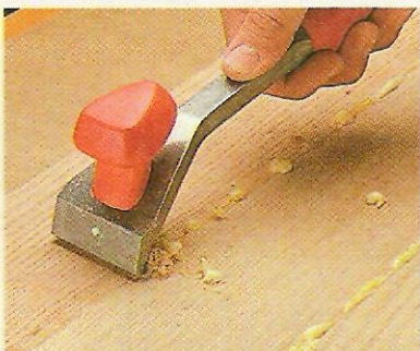
4 Remove Excess. Finally, remove the dried "foam" by scraping (shown above left) or sanding. Removing glue from hard-to-reach areas like a corner (photo at right) is a snap with a sharp chisel — it "pops" right off.
