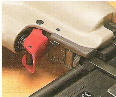
▲ Depth Adjustment. A mechanical depth adjustment like a thumb screw (left) or sliding tab (right) makes fine tuning how deep the nail is set easier than having to modulate the amount of air coming from the compressor.
