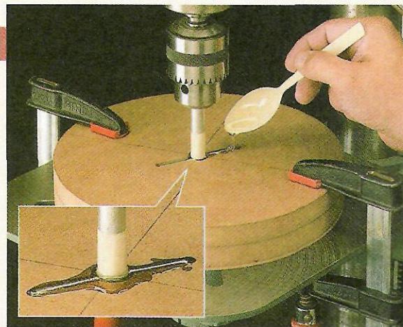
▲ Adding the Epoxy. Carefully spoon the epoxy all around the shaft and cross pin, letting it ooze into the "well" created by the counterbore. You can temporarily mask off the shaft with a piece of tape.
