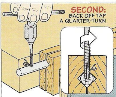
Step 5. With the tap straight up and down, begin cutting the threads (left). After each half-turn, back off the tap a quarter-turn to clear the waste (right). Then just repeat the process until the threads are cut all the way through.
