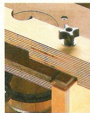
▲ Fence. This adjustable fence slides in the T-slots on the router base plate.
