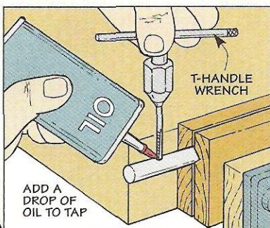
Step 4. Now position the tap so it's straight up and down. Then add a few drops of oil to the tap threads.
