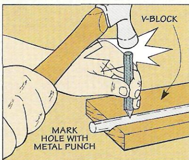
Step 1. To prevent the bit from wandering, use a metal punch to create a dimple in the rod.
