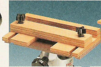
MORTISING JIG
