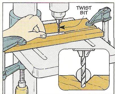
Step 2. Start by drilling a small hole. Then increase the hole size using progressively larger drill bits.
