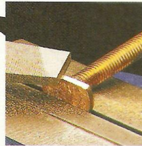
▲ T-Bolts. Lightly file down the sides of the toilet bolts so they slide smoothly in the slots.
