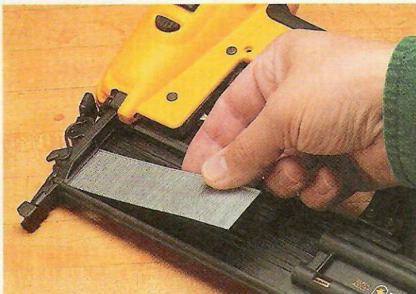
▲ Loading. Loading brad nails is easy and convenient. Just release the magazine, lay a clip inside (above), and then slide the magazine forward to lock it in place.
