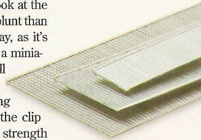
▲ Nail Sizes. Most brad nailers will handle a wide range of nail lengths, but often in two different ranges — \frac{3}{8} " to 1\frac{1}{4} " or \frac{5}{8} " to 2".
