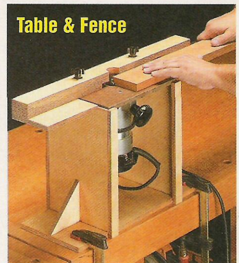
Mortising Jig
