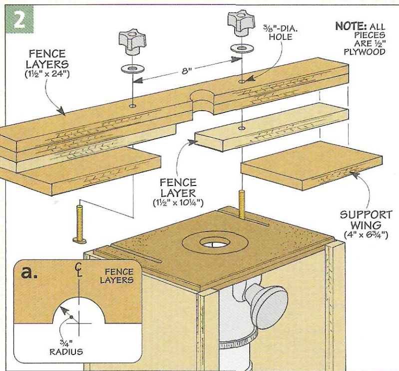
▲ Fence. This adjustable fence slides in the T-slots on the router base plate.
