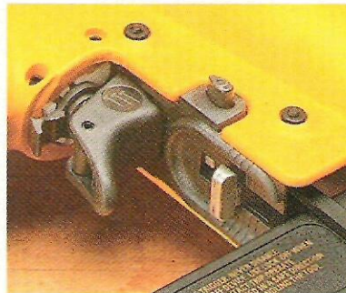
▲ Depth Adjustment. A mechanical depth adjustment like a thumb screw (left) or sliding tab (right) makes fine tuning how deep the nail is set easier than having to modulate the amount of air coming from the compressor.
