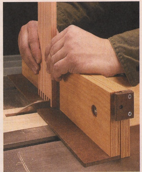
Box Joint Jig
