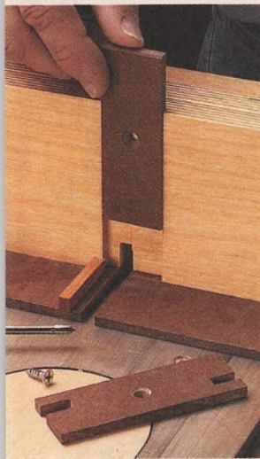
▲ Replaceable Insert. A hardboard backing insert can be easily replaced as it gets chewed up through use.
