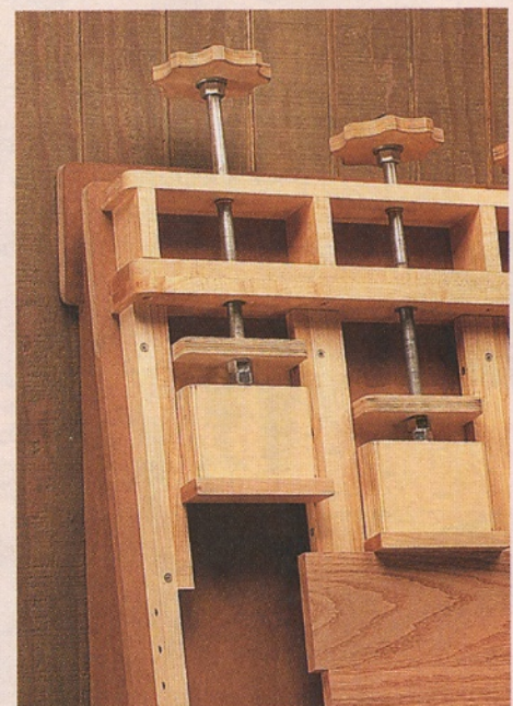
Clamping Station
