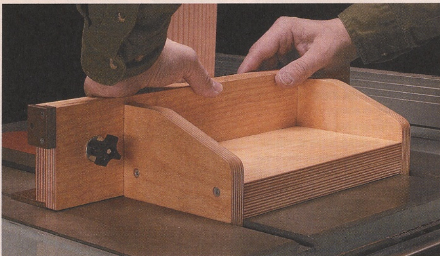
▲ Two are Better Than One. The sides of this jig form runners that ride in the miter gauge slots of your table saw.
