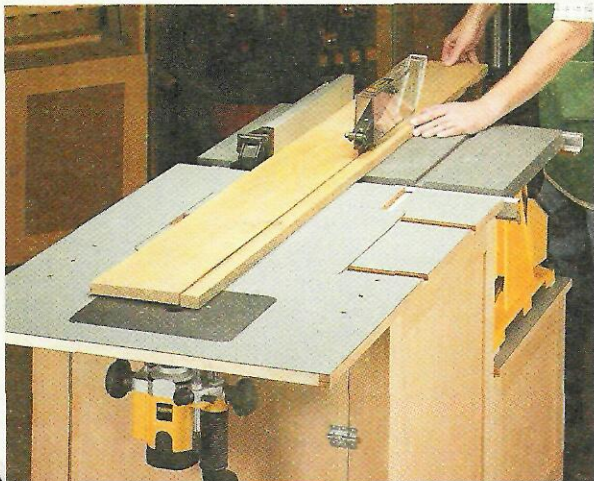
A. Convertible Top. Positioning the top so it extends over the back of the outfeed cabinet creates a long, stable support surface when ripping long workpieces.
