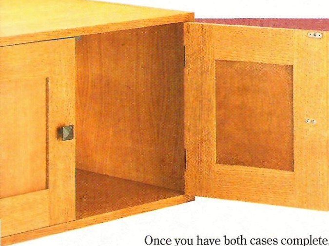
▲ Open and Shut Case. A pair of hinged doors open to reveal a large storage compartment.
