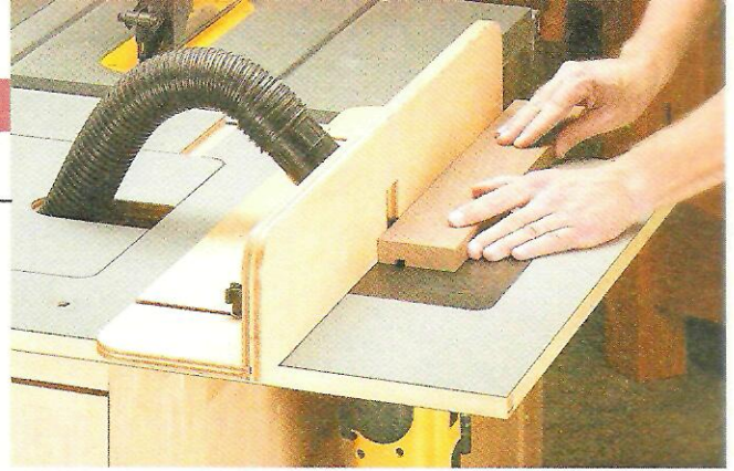
▲ Fence. Adding a fence to the router table adds versatility and allows you to hook up the hose from the shop vacuum.
