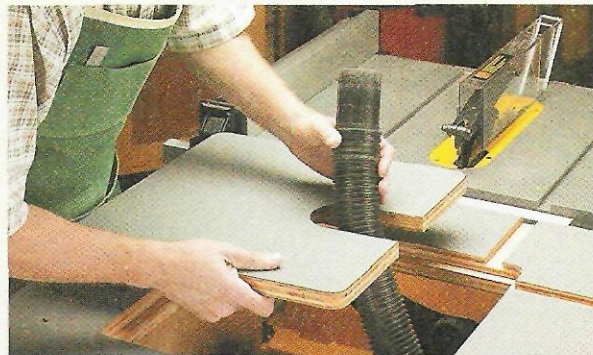
B. Shop Vacuum Access. A removable panel provides quick access when hooking the dust hose from the shop vacuum up to the table saw or router table fence.
