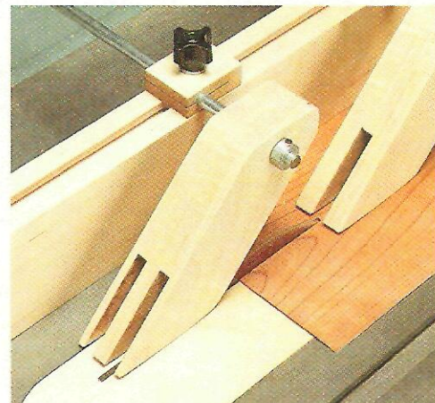
▲ Added Control. Using this jig with a zero-clearance insert on your table saw will give you greater control and accuracy when cutting thin laminates and veneers.
