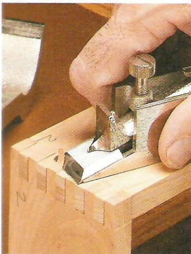
▲ Chisel Plane. With the top removed, this plane is quickly converted into a chisel plane. The low-angle blade cuts right through the end grain on this box joint.
