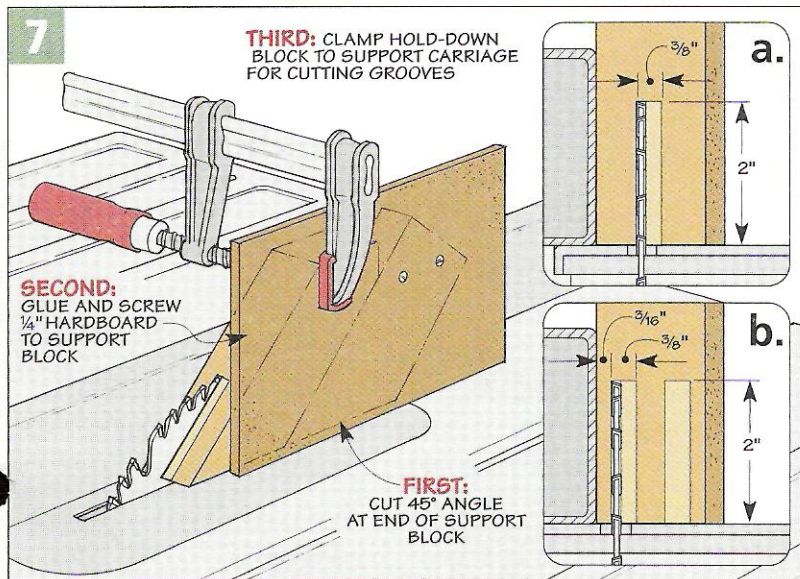
▲ Added Control. Using this jig with a zero-clearance insert on your table saw will give you greater control and accuracy when cutting thin laminates and veneers.
