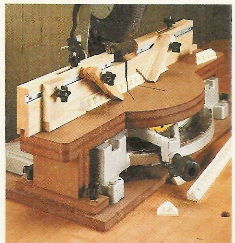
Miter Saw Table & Fence page 6
