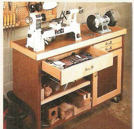
Mini-Lathe Stand page 14
