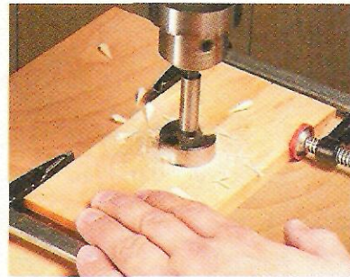
◀ Finger Openings. Clamping a pair of drawer fronts together provides solid support when drilling the circular cutouts for the finger openings.
