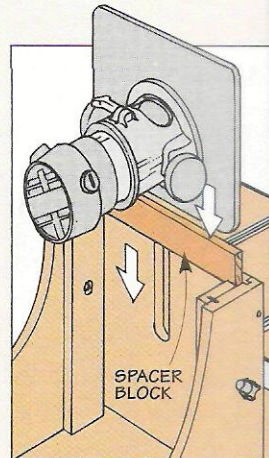
▲ Spacer Block. The router plate rests on a spacer block. By using different widths of blocks, you can vary the height of the router for different thicknesses of stock.
