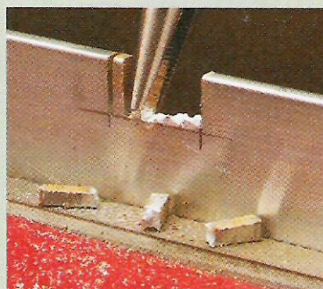
▲ Snap. Using a pair of needle-nose pliers, snap off the remaining waste pieces one by one.
