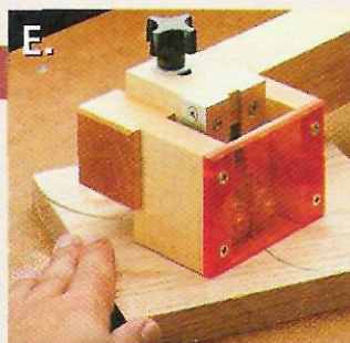
▲ Polycarbonate & Acrylic. Virtually unbreakable, polycarbonate is best for see-through guards (left) while inexpensive acrylic makes a great hairline indicator (right).
