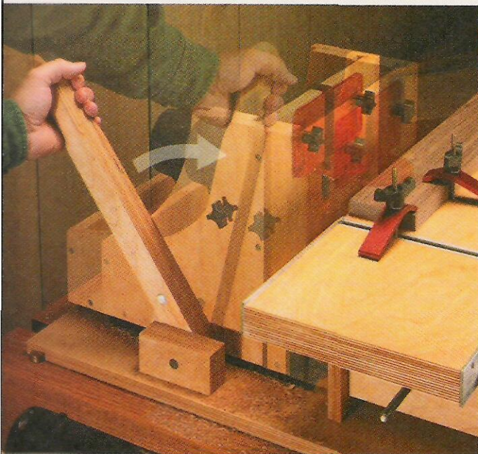
▲ Lever Arm. The carriage travels on a pair of drawer slides. A lever arm is used to move the carriage forward or backward.
