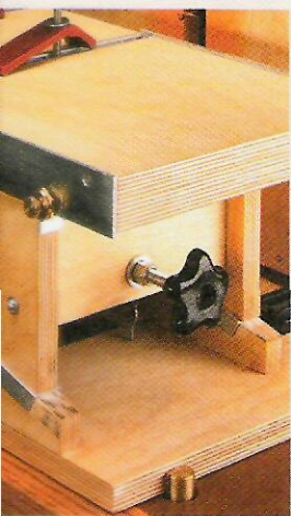
▲ Height Adjustment. Turning a knob at the end of the tapered bed will raise or lower the sliding table.
