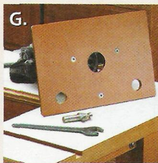
▲ Phenolic & Laminate. A phenolic plate is the perfect choice for mounting a router (left). And laminate makes a long-wearing and easily replaceable platen for an edge sander (right).
