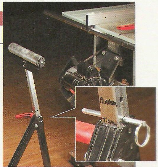
▲ Mark McConnel of Costa Mesa, CA quickly sets the height of his outfeed rollers by drilling holes in the riser and locking it in place with a hitch pin.
