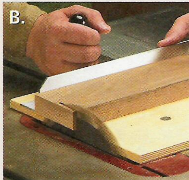
▲ Plywood. A mainstay for long-lasting jigs, high-quality plywood (like the Baltic birch shown above) provides flatness and stability for fences (left) and bases (right).
