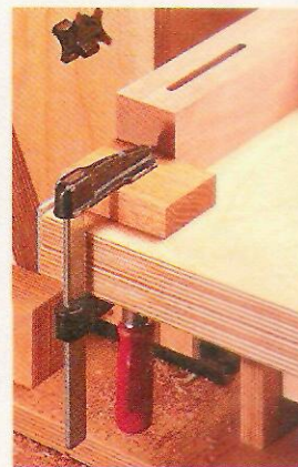
▲ Stop Block. To rout mortises in multiple workpieces, clamp a simple stop block to the sliding table to position all the pieces the same.
