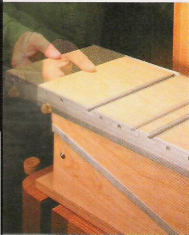
▲ Sliding Table. To rout a mortise, the table slides from side to side on the tapered bed.
