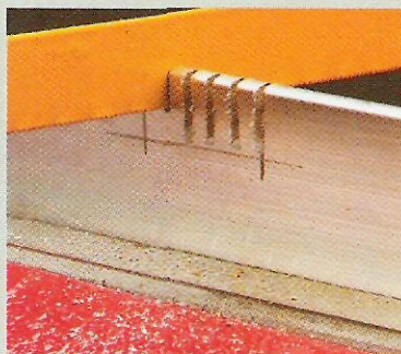
▲ Cut. To create the notches for the T-track, start by cutting a row of kerfs with a hack saw.
