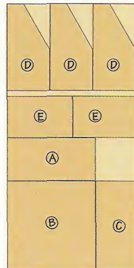
CUTTING DIAGRAM
