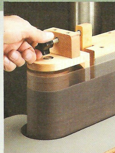
▲ Tracking. Turning a knob at the end of the sander will cause the idler roller to pivot slightly, thereby centering the belt.
