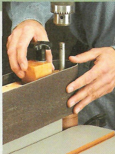
▲ Belt Change. To install or remove the sanding belt, loosen the knob and lift up the wedge to release the tension on the sanding belt.
