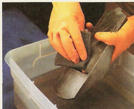
3 Once the electrolysis is complete, rinse the tool off in clean water and scrub the surfaces gently with the abrasive pad.
