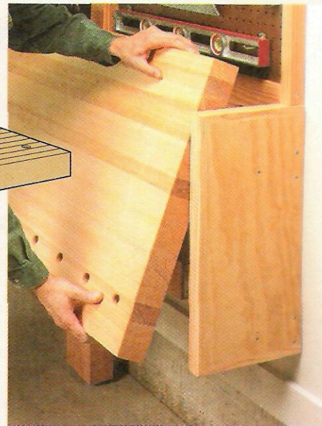
▲ Space-Saving Design. The top of the workbench folds down against the base to save space when you're not using it.
