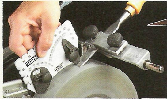
◀ Set the Angle. With the AngleMaster, you can verify (see inset) and set the sharpening angle perfectly.
