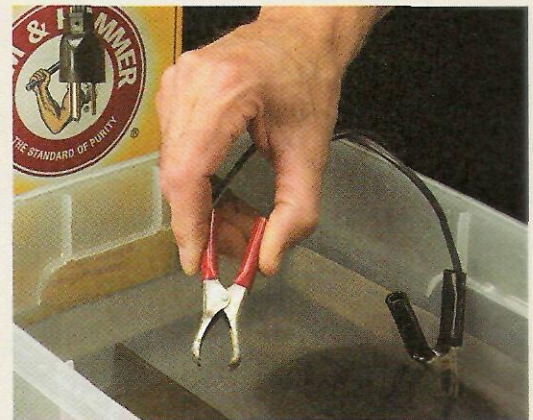
2 With the battery charger unplugged, clamp the negative lead to the tool and the positive lead to the anode (a scrap piece of steel).
