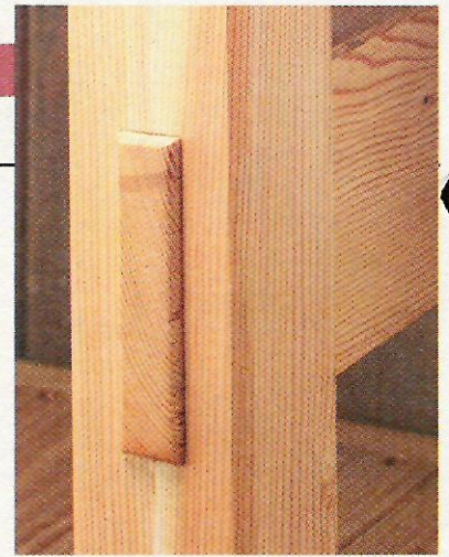
▲ Through Tenons. A few cuts on the table saw are all it takes to make perfectly sized mortises for the through tenons of the bench.
