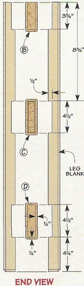
▲ Through Tenons. A few cuts on the table saw are all it takes to make perfectly sized mortises for the through tenons of the bench.
