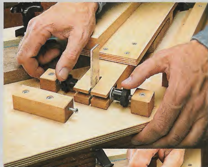
▲ Plus or Minus 45° Cuts. Whenever you need to cut an angle greater or less than 45° to square up a miter joint, simply lift up the aluminum guide stop. Then adjust the two knobs to change the miter angle for trimming.
