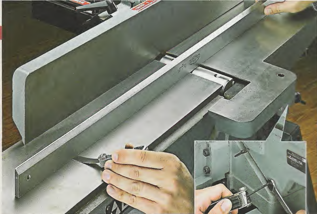
▲ Checking the Alignment. A precision straightedge and feeler gauge allow you to check whether the outfeed table sags (top). Snugging up the gib may help remove the sag (inset).
