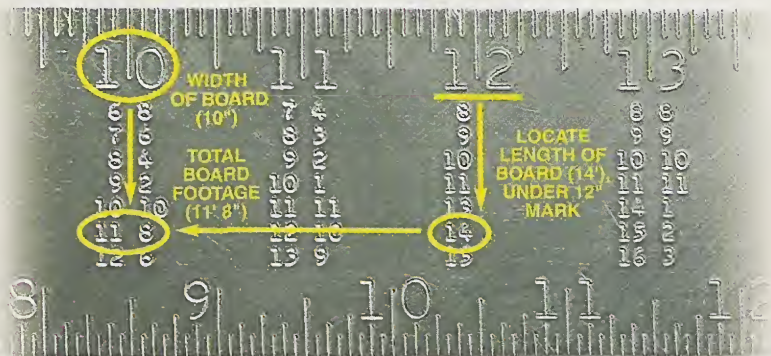
▲ Board Footage Table. By using this table (usually found on the back of the blade) you can determine the number of board feet in a given piece of lumber (in this example, a board that is 14' long and 10" wide).
