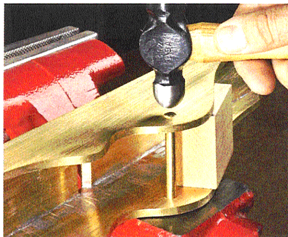
▲ Add the Pin. Cut the brass rod for the cross pin a hair longer than needed and peen the ends over with a hammer. Then file and sand the ends of the pin flush with the surface of the sides of the plane.
