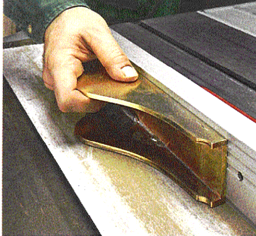
▲ Square it Up. To clean up the outside of the plane and square the sides with the sole, place a piece of adhesive-backed sandpaper on the top of your table saw.
