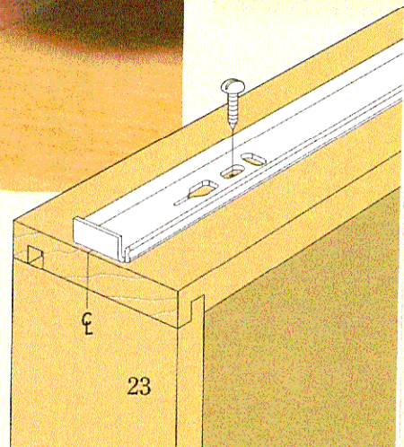
▲ Installing Slides. A scrap of plywood makes it easy to level a drawer slide. The other half of the slide is centered on the drawer side and screwed in place (right).
