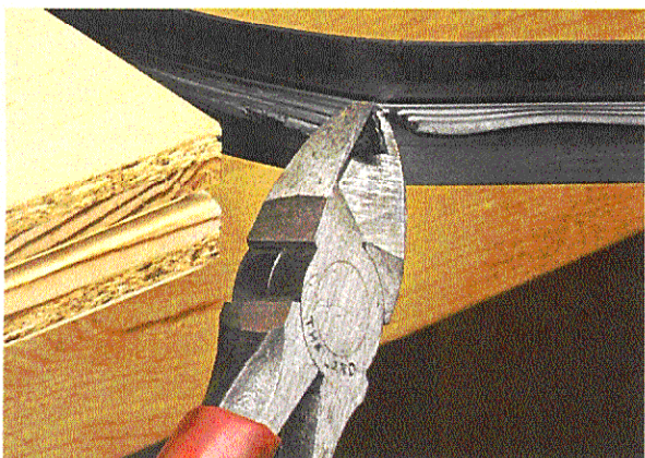
▲ Notch It. Fitting the molding around a 90° corner requires a notch. I used flush-cutting pliers to cut a small V-shaped piece from the barbed section.
