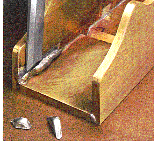
▲ Cleaning the Inside. An old chisel comes in handy to remove any globs of solder from inside the body of the plane. Then you can scrape or sand away any remaining traces.
