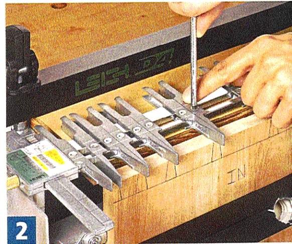
2 Adjust the Fingers. Using the tail board as a guide, adjust the fingers to match nearly any layout you can come up with.
