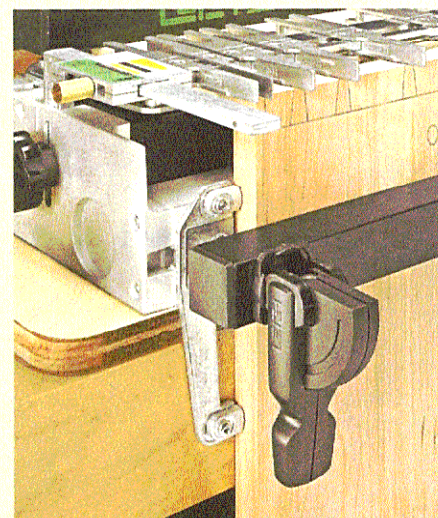
Cams & Stops. Adjustable cams lock the workpiece securely in place and adjustable stops ensure the workpiece is positioned properly.
