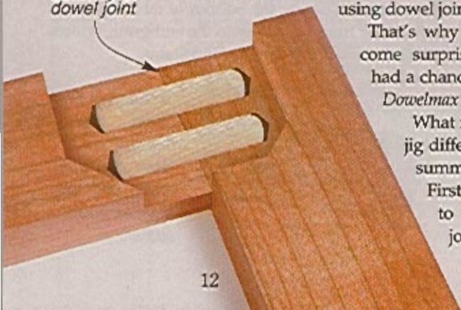
Cutaway of dowel joint
