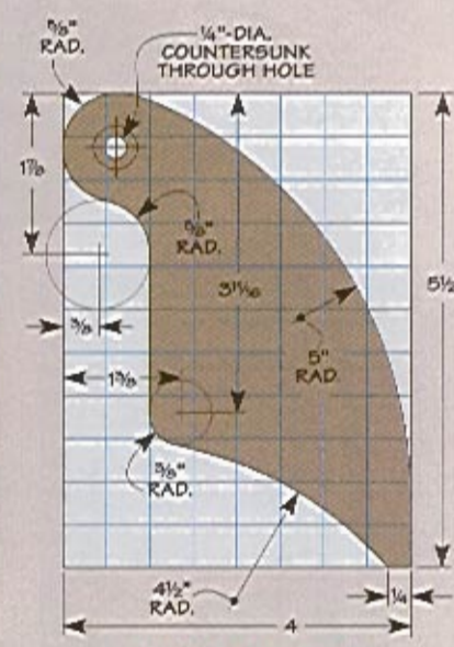
GUARD PROFILE
