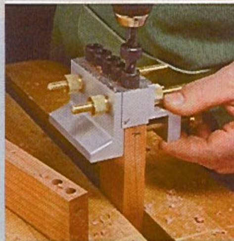
▲ Matching Holes. To drill matching holes in the end of the mating piece, you repeat the process. The jig is clamped flush with the marked edge of the workpiece.
