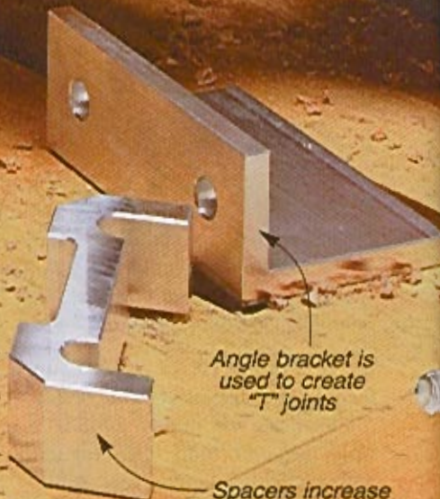
Spacers increase capacity and are used to make offset joints
