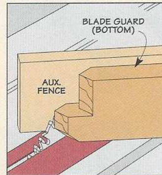
▲ Compound Cut. The last set of cuts is on the top of the blade guard. Tilt the saw blade 45° and cut the remaining bevels from the nose.
