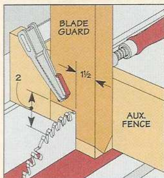
▲ The First Cut. Using an auxiliary fence on your miter gauge, start forming the notches for the permanent fences in the blade guard.
