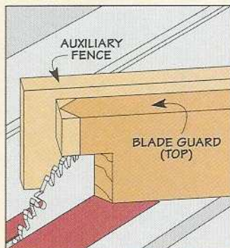
▲ Miter for the Fences. Rotate your miter gauge 45° to complete the notches where the fences will rest. Make two cuts to center the point.
