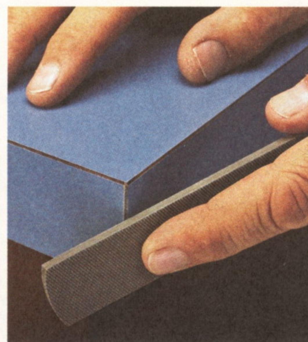
▲ Filing Edges. Downward and outward strokes of a flat mill file make smooth edges.
