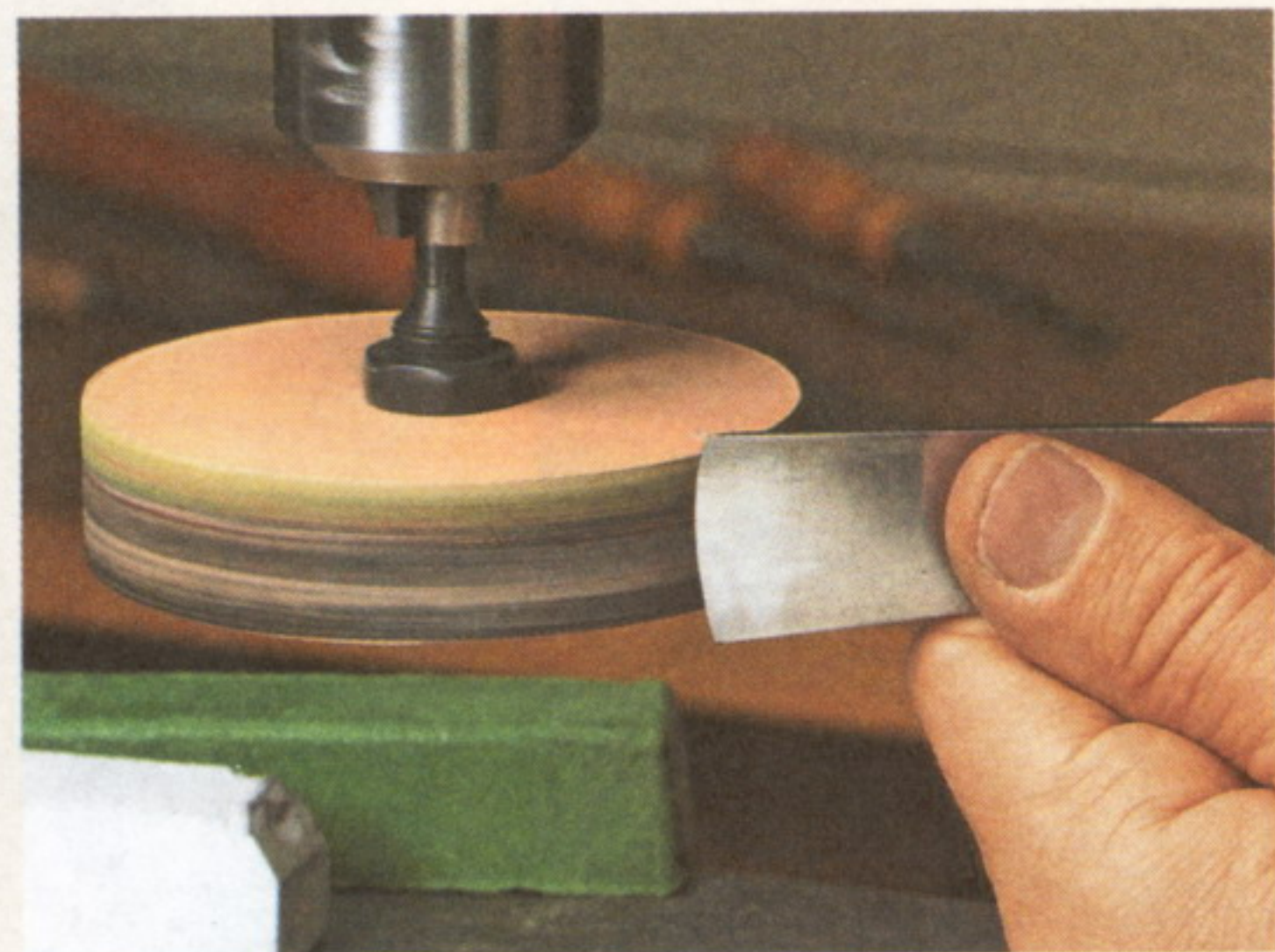
▲ Buffing Wheel. A wheel charged with different grades of abrasive compound can polish the edge of a gouge in no time.
