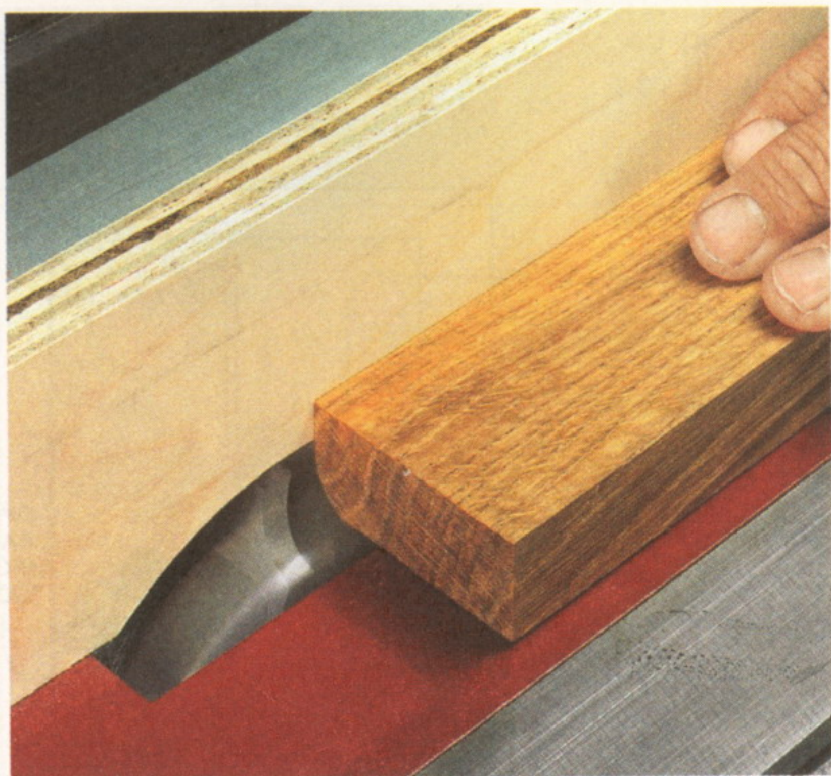
▲ Auxiliary Fence. Burying the knives in an auxiliary rip fence allows you to shape the edge of a board using just a portion of the knife profile.
